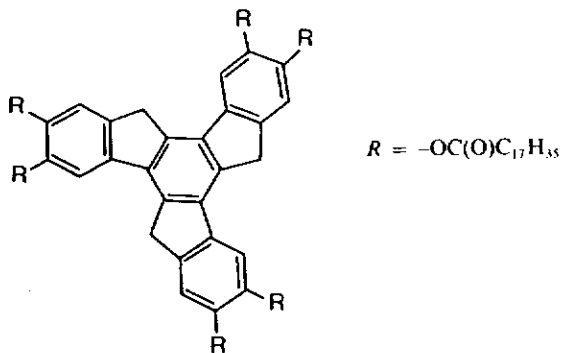
Figure 1. Structure of 2,3,7,8,12,13-hexa(octadecanoyloxy)truxene.
