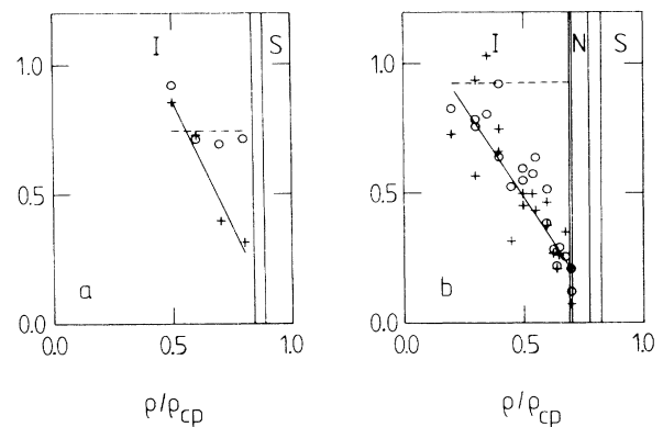
FIG. 2. Density dependence of the ratio of single-particle to collective times \tau_2^i/\tau_2^c (pluses) and the contribution (1 + g_2)^{-1} (circles). We show a linear least-squares fit to \tau_2^i/\tau_2^c (solid line) and the average value of 1 + j_2 (dashed line). The isotropic (I), nematic (N), and solid (S) regions are indicated, with two-phase regions delimited by vertical lines. (a) a/b=2 , (b) a/b=3 .
