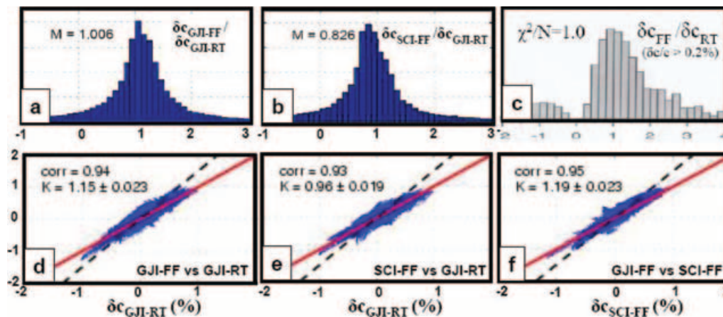
Figure 6. Comparison of wavespeed perturbations \delta c inferred from FFT and RT inversions by means of histograms and scatter plots. We use \delta c_{\text{GJI-FF}} , \delta c_{\text{GJI-RT}} , and \delta c_{\text{SCI-FF}} to denote the relative variation in wavespeed according to the PRI-GJI-FFT, PRI-GJI-RT, and PRI-SCI-FFT models, respectively. Unless noted otherwise, we compare the models at a depth of 1350 km in the mantle. (a) histogram of \delta c_{\text{GJI-FF}}/\delta c_{\text{GJI-RT}} (the average value of this distribution is \sim 1 ); (b) histogram of \delta c_{\text{SCI-FF}}/\delta c_{\text{GJI-RT}} (the average ratio is \sim 0.83 ); (c) histogram of \delta c_{\text{FF}}/\delta c_{\text{RT}} for a depth of 1450 km, for values |\delta c/c| larger than 0.2 per cent, and for models with \chi^2/N = 1.0 (after fig. 13 of M04a) (according to M04a the mean of this distribution is around 1.7). The low count near zero, the skewness of the main lobe, and the large averages all result from omitting low values of |\delta c/c| from the analysis. (d) Scatter plot of \delta c_{\text{GJI-FF}} vs. \delta c_{\text{GJI-RT}} : the correlation coefficient, R , is 0.94; the slope (from bi-variant regression) is 1.15, with an uncertainty of 0.023 (based on an assumed error in \delta c/c of 0.2 per cent); (e,f) Same for \delta c_{\text{SCI-FF}} vs. \delta c_{\text{GJI-RT}} ( R = 0.93 , slope = 0.96) and \delta c_{\text{GJI-FF}} vs. \delta c_{\text{SCI-RT}} ( R = 0.95 , slope = 1.19), respectively. The dashed line (slope of 1.5) would be consistent with a \sim 50 per cent amplitude increase.
