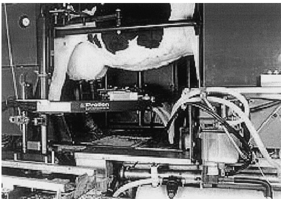
Fig. 1. A Milking robot. (Source: IMAG-DLO)
