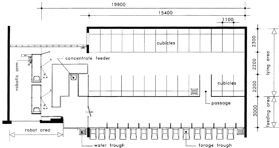
Fig. 2. Layout of the experimental barn in Duiven. Dimensions in mm. (Source: IMAG-DLO)
