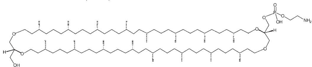
(r) Di-glycerol tetraether phospholipids (caldarchaeols): sn -caldarchaeo-1-phosphoethanolamine
