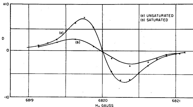
FIG. 5. Plot of the reading of the output meter M_s , for a 0.5N solution of ferric nitrate. Curve (b) was taken at a high power level and shows the effect of saturation. The value of the magnetic field at the line center was not measured, but merely computed from the frequency and the accepted value of the proton moment.
