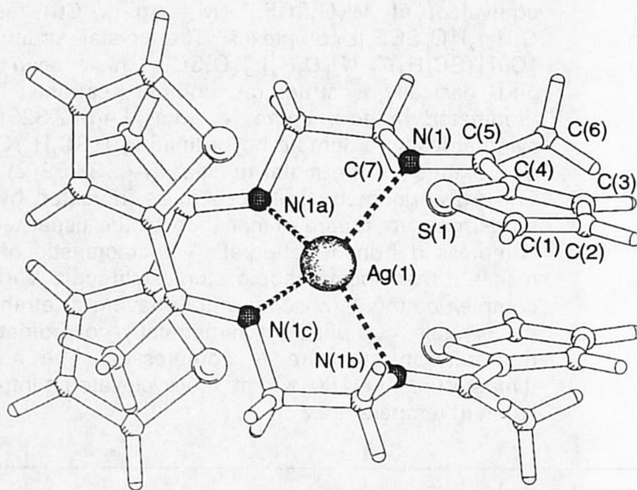
Fig. 1 A PLUTON 8 drawing of [Ag\{[(SC_4H_3)CMe=N]_2C_2H_4\}_2]^+ with the atom labelling scheme
