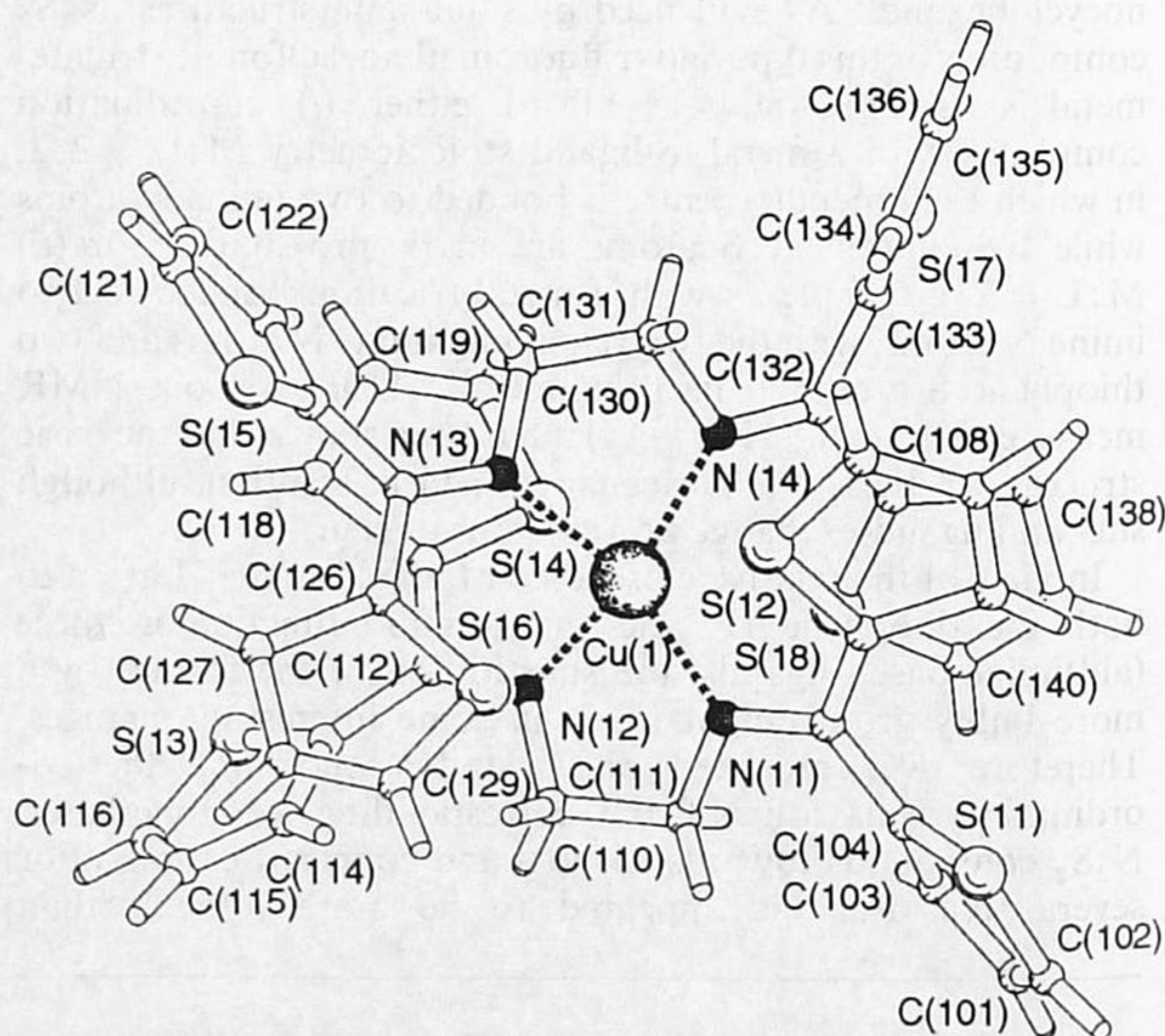
Fig. 2 A PLUTON 8 drawing of [Cu\{[(SC_4H_3)_2C=N]_2C_2H_4\}_2]^+ (molecule 1) with the atom labelling scheme
