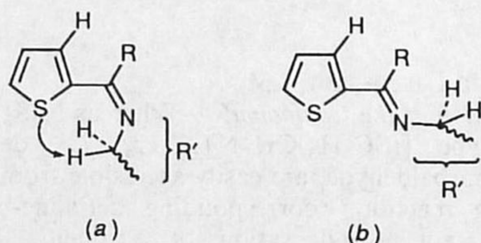
Scheme 1 The S=C-C=N sym-cis conformation with (a) Z and (b) E C=N configuration
