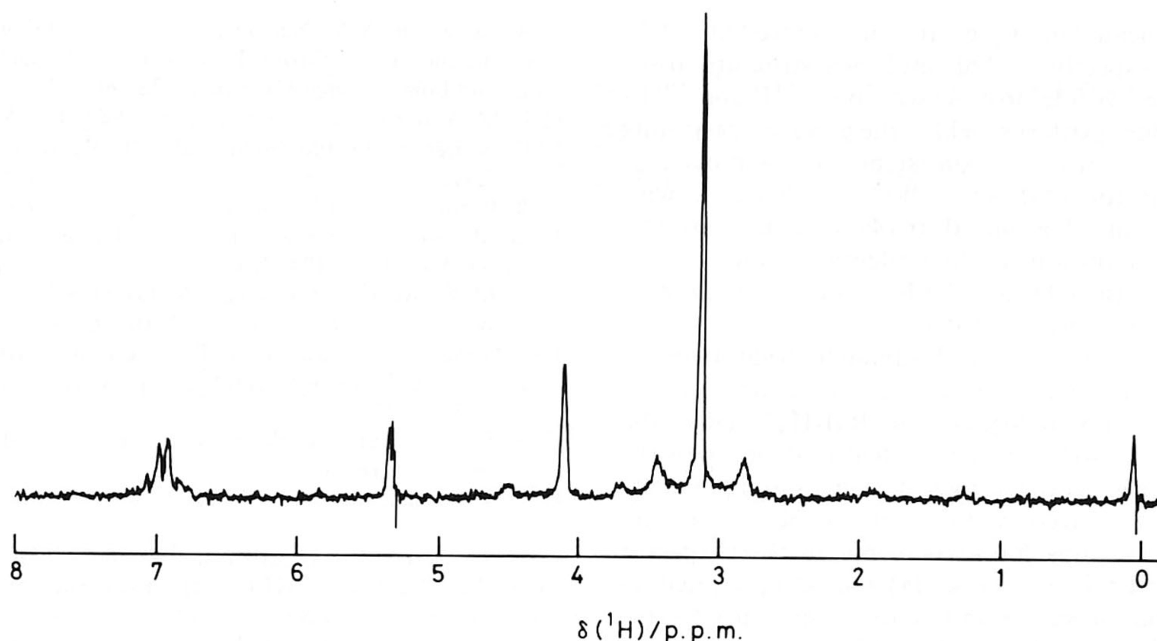
Figure 4. 60-MHz ^1\text{H} n.m.r. spectrum of [(\text{L}^1)\text{Pt}(\mu\text{-Cl})\text{Pt}(\text{L}^1)]\text{BF}_4 ( 1a )
