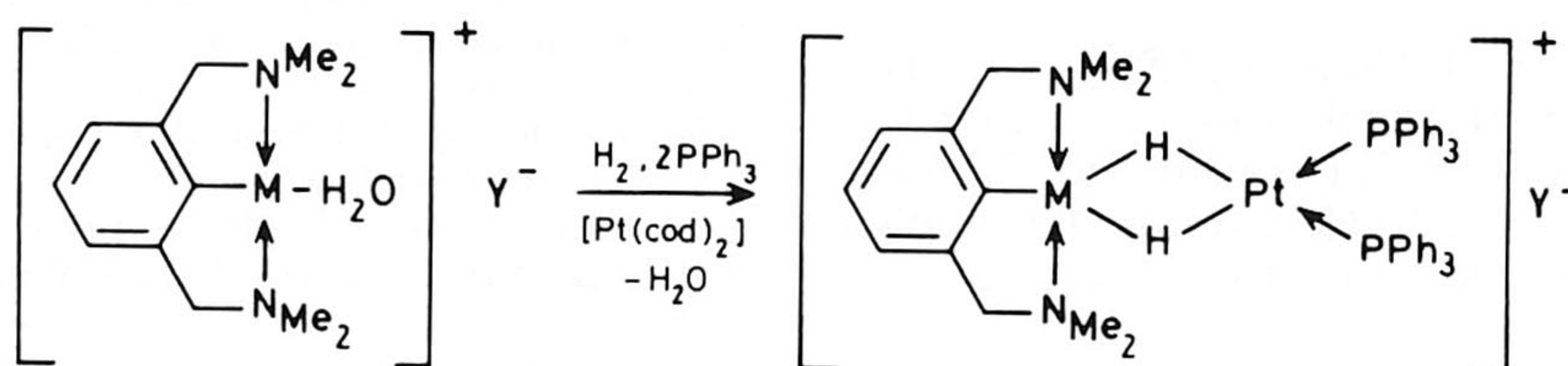
Scheme 2. Synthesis of the bimetallic dihydride complexes: \text{M} = \text{Pt} , \text{Y} = \text{BF}_4 ( 4a ), \text{M} = \text{Pd} , \text{Y} = \text{BF}_4 ( 4b )
