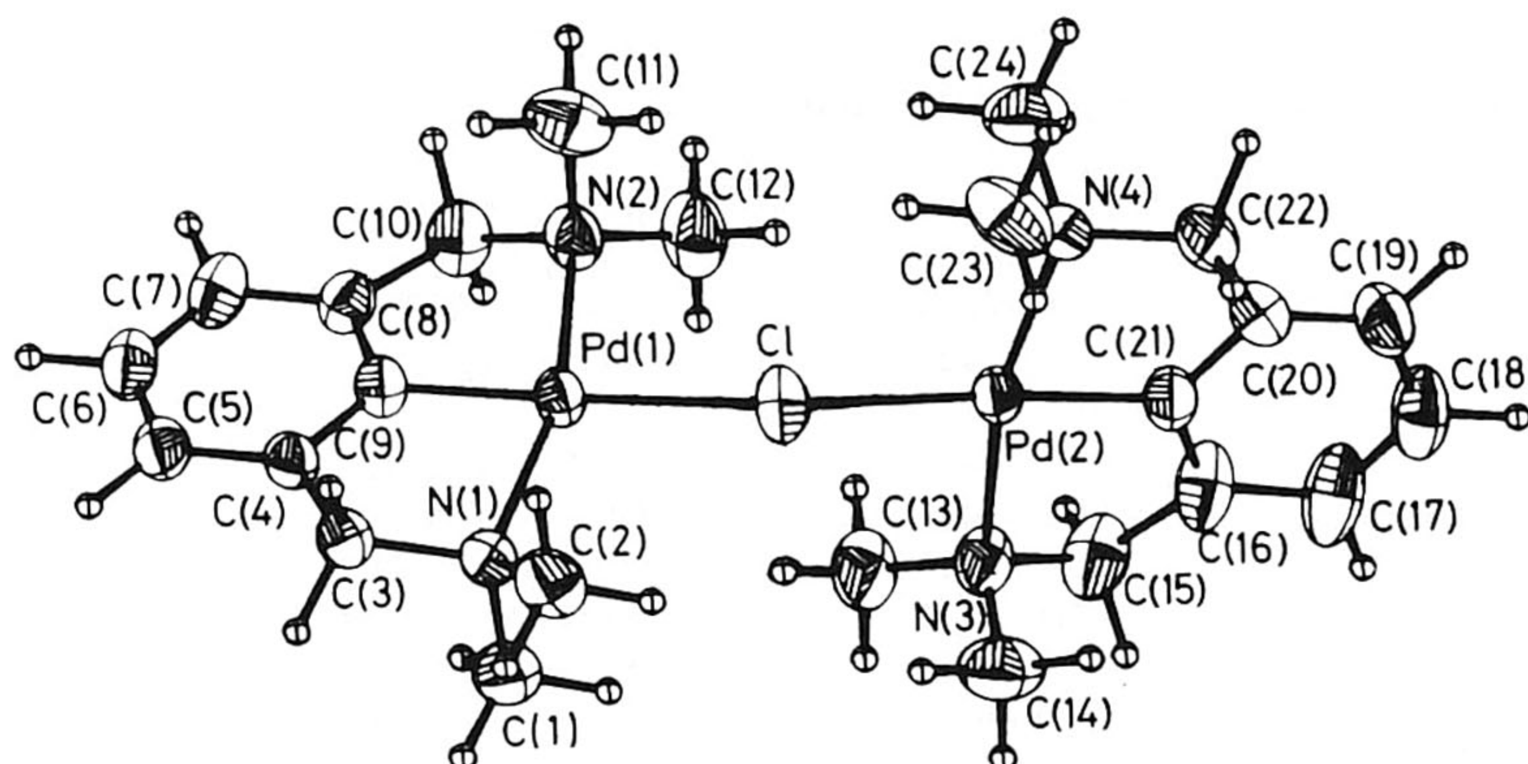
Figure 2. ORTEP drawing of [(L^1)Pd(\mu\text{-Cl})Pd(L^1)]BF_4 ( 2a ) with numbering scheme (40% probability). The hydrogen atoms are represented by artificially small spheres. The BF_4^- anion is shown in Figure 1
