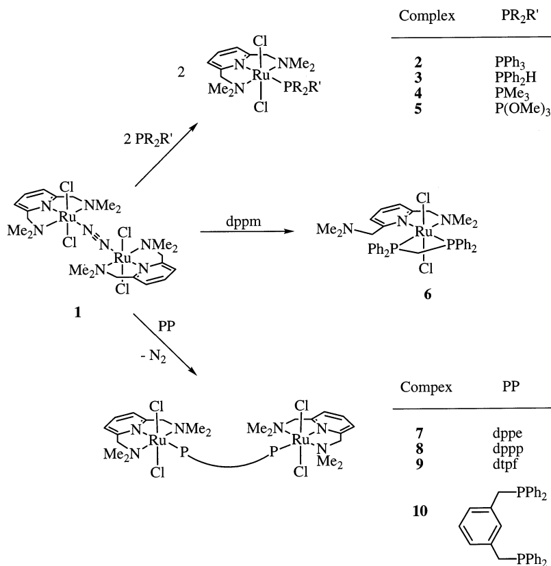
Fig. 1. dppm, 1,1'-bis(diphenylphosphino)methane; dppe, 1,2-bis(diphenylphosphino)ethane; dppp, 1,3-bis(diphenylphosphino)propane; dtpf, 1,1'-bis[di( p -tolyl)phosphino]ferrocene.
