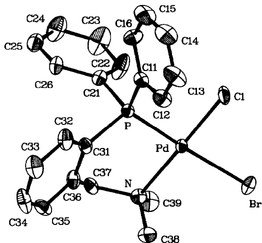
Fig. 1. Molecular structure of \text{Pd}(\text{Me})(\text{Br})(\text{PN}) ( 6b ) with adopted numbering scheme.
