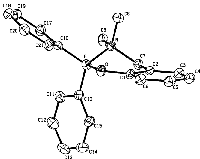
Fig. 1. Displacement ellipsoid plot of 2 , drawn at 50% probability. Hydrogen atoms are omitted for clarity.
