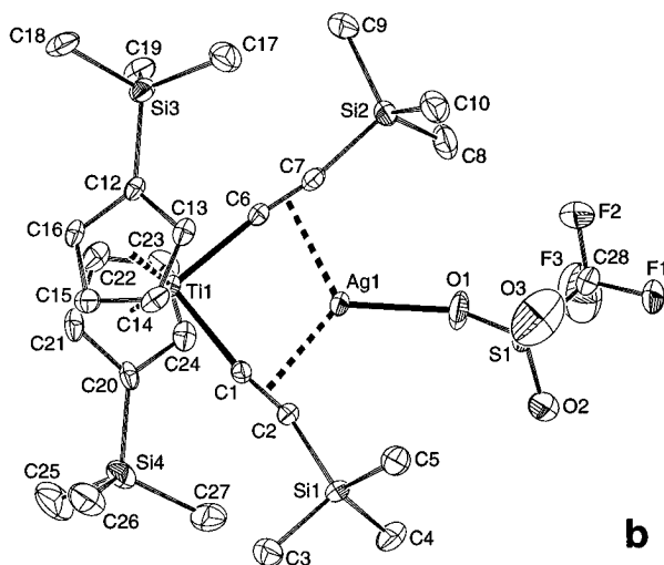
Figure 2. ORTEP drawings (drawn at the 30% probability level) of the complexes [(\eta^5\text{-C}_5\text{H}_4\text{SiMe}_3)_2\text{Ti}(\text{C}\equiv\text{CSiMe}_3)_2]\text{MOSO}_2\text{CF}_3 (with the exclusion of the hydrogen atoms) with the adopted atom-labeling scheme: (a) \text{M} = \text{Cu} ( 2 ); (b) \text{M} = \text{Ag} ( 3 ).
