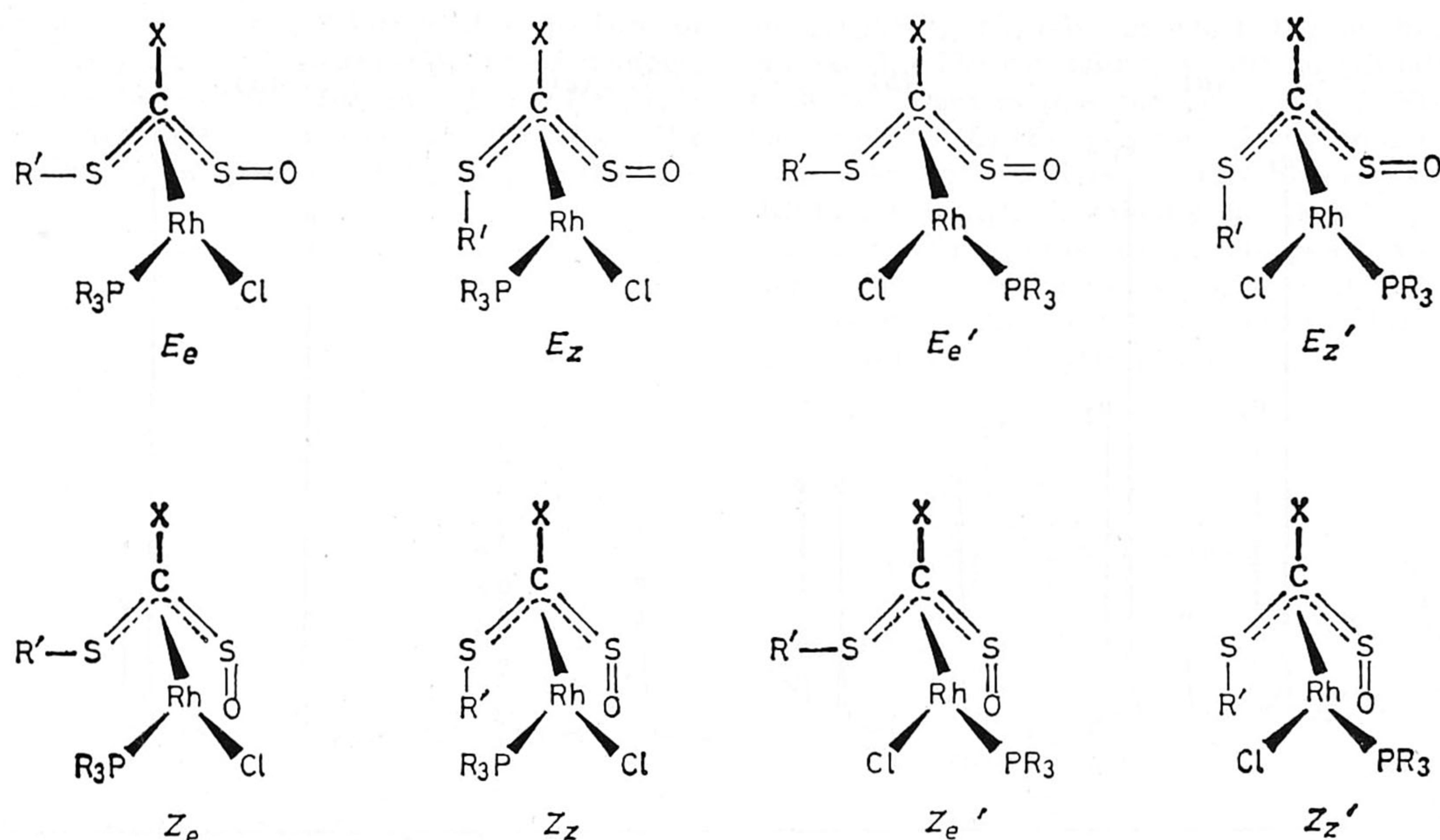
FIGURE 2 Four possible structures for [\text{Rh}^{\text{I}}\text{Cl}(\text{PR}_3)\{(E)\text{-}(\text{MeS})(p\text{-MeC}_6\text{H}_4)\text{CSO}\}] and [\text{Rh}^{\text{I}}\text{Cl}(\text{PR}_3)\{(Z)\text{-}(\text{MeS})(p\text{-MeC}_6\text{H}_4)\text{CSO}\}] ( E - and ( Z )- (2b ; R = \text{C}_6\text{H}_{11} ), (3b ; R = \text{Pr}^i ) and [\text{Rh}^{\text{I}}\text{Cl}(\text{PR}_3)\{(E)\text{-}(\text{R}'\text{S})_2\text{CSO}\}] and [\text{Rh}^{\text{I}}\text{Cl}(\text{PR}_3)\{(Z)\text{-}(\text{R}'\text{S})_2\text{CSO}\}] ( E - and ( Z )- (2c ; R = \text{C}_6\text{H}_{11} , R' = p\text{-MeC}_6\text{H}_4 ), (2c' ; R = \text{C}_6\text{H}_{11} , R' = \text{Ph} ), (3c ; R = \text{Pr}^i , R' = p\text{-MeC}_6\text{H}_4 )
