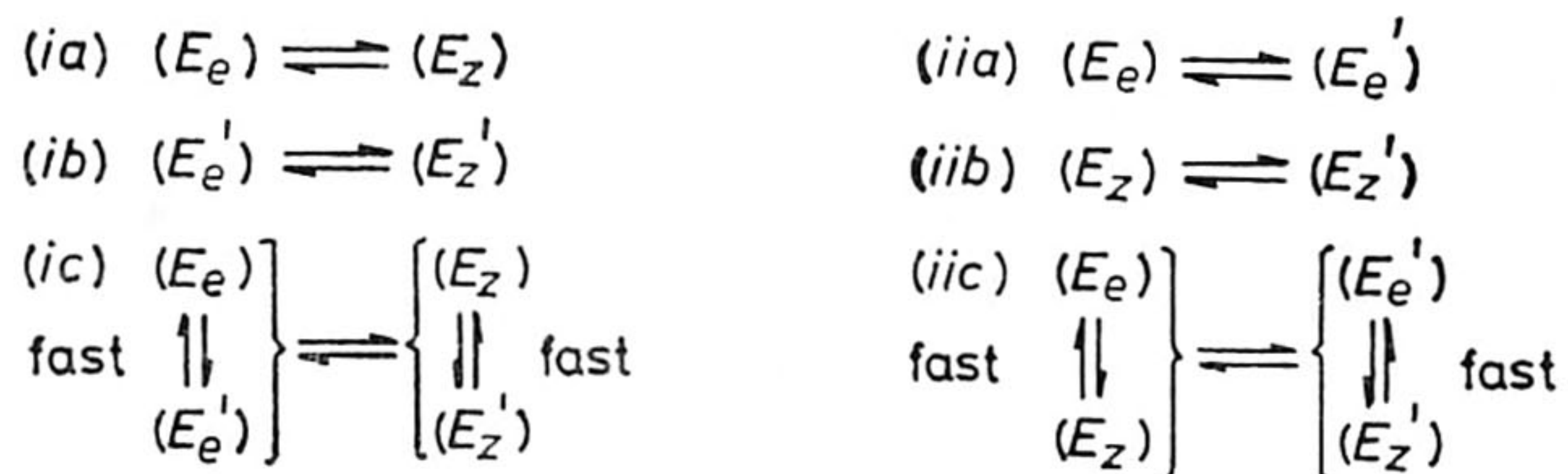
SCHEME The possible fluxional processes
