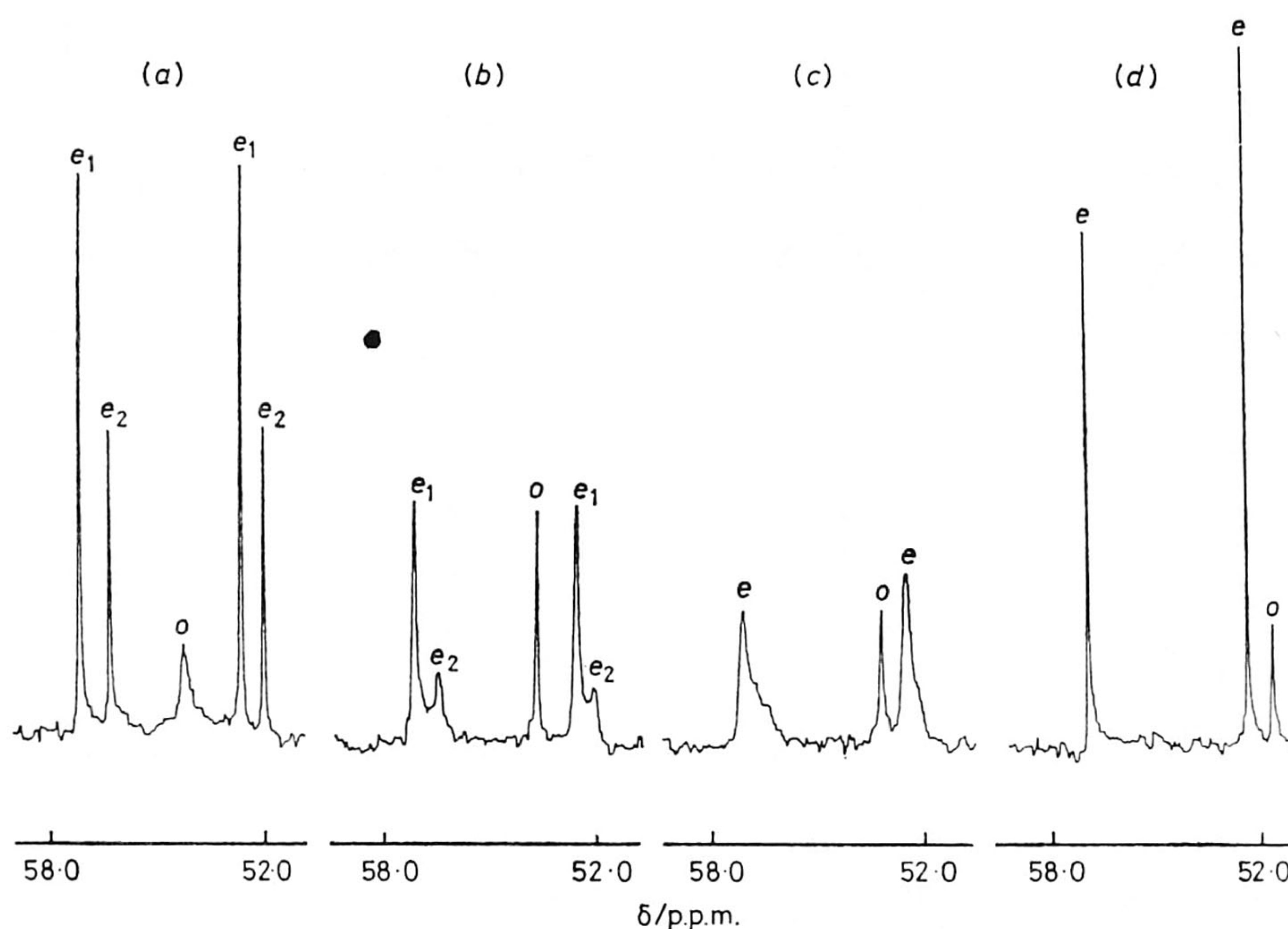
FIGURE 3 Phosphorus-31 n.m.r. spectra recorded on a C_6D_5CD_3 solution of [Rh^I Cl\{P(C_6H_{11})_3\}\{(E)-(MeS)(p-MeC_6H_4)CSO\}] ( E )-(2b) at -46.5 (a), -6.5 (b), 3.5 (c), and 48.0 °C (d); e_1 and e_2 refer to ( E )-(2b) in slow exchange, e to ( E )-(2b) in fast exchange, and o to P(C_6H_{11})_3O
