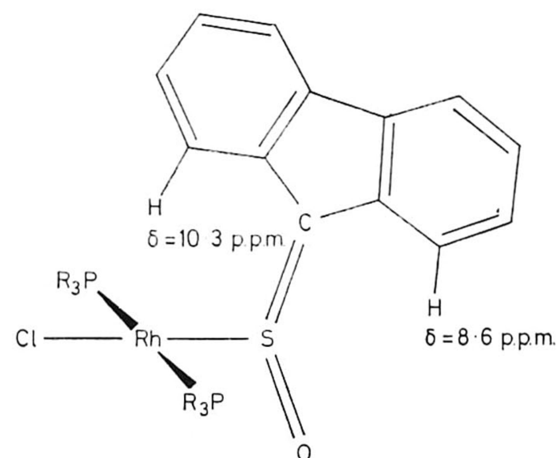
FIGURE 1 Structure of trans - [\text{Rh}^{\text{I}}\text{Cl}(\text{PR}_3)_2(\text{C}_{12}\text{H}_8\text{CSO})] ( \text{R} = \text{C}_6\text{H}_{11} or \text{Pr}^i ) (4a) and (5a)
