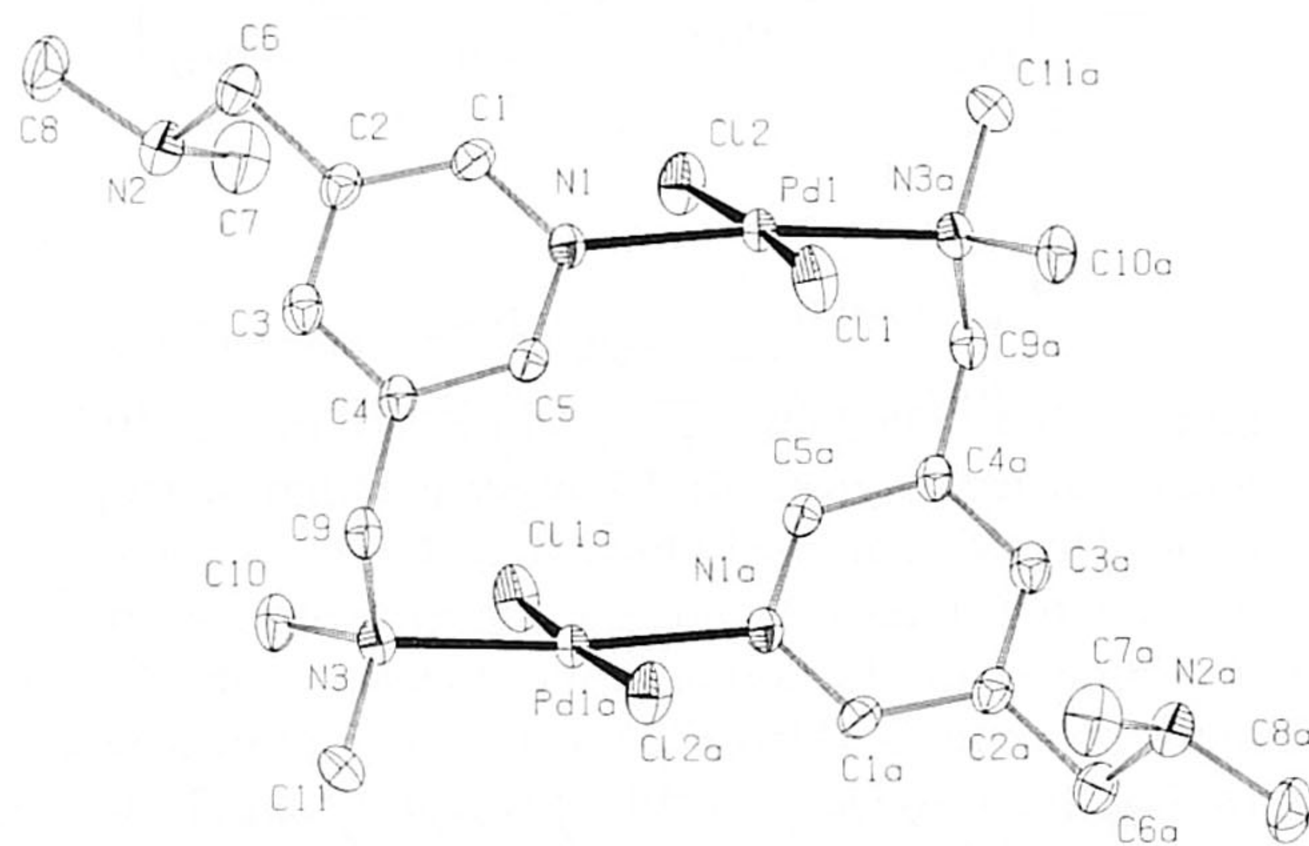
Figure 1. An ORTEP diagram (50-% probability level) of the molecular structure of complex 4 showing the adopted numbering scheme
