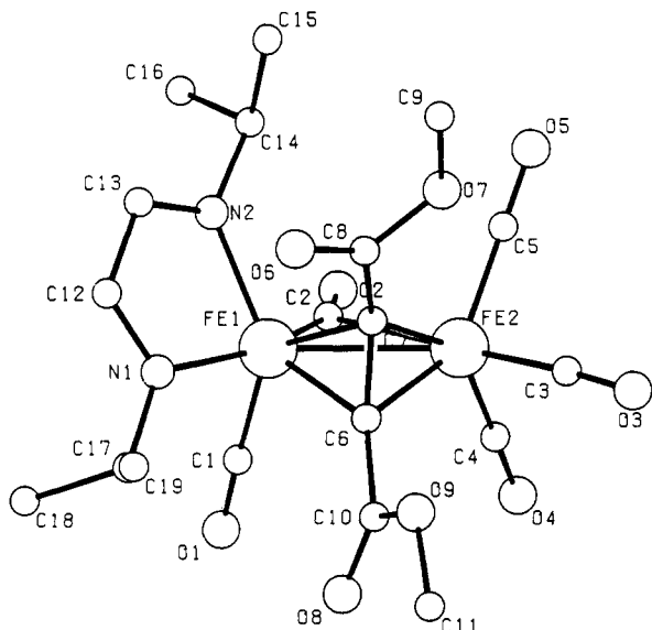
Figure 1. PLUTO drawing of \text{Fe}_2(\text{CO})_5(i\text{-Pr-DAB})[\mu_2, \eta^2\text{-MeOC(O)C}\equiv\text{CC(O)OMe}] (3).
