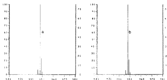
Figure 4. Observed (a) and calculated (b) mass spectra of [\text{FeMn}(\text{CO})_6(\text{t}-\text{Bu}-\text{AAA})] .
