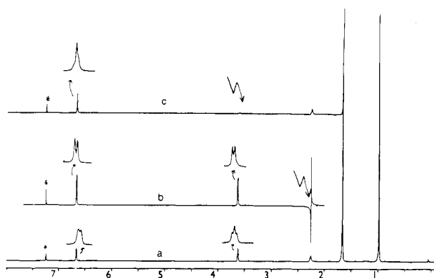
Figure 5. a: Normal ^1\text{H} NMR spectrum of [\text{FeMn}(\text{CO})_6(\text{t-Bu-AAA})] . b: Irradiated at N-H (2.3 ppm). c: Irradiated at C(8)-H(8) (3.6 ppm) (the asterisk is CHCl 3 ).
