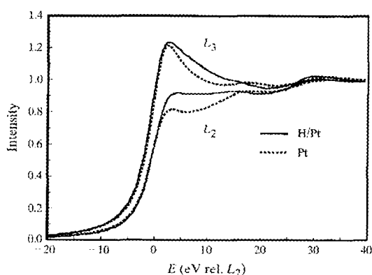
Figure 2 L_3 and L_2 near-edge spectra for H—Pt/Sap6 (reduced at 673 K, hydrogen chemisorbed, solid line) and Pt/Sap6 (evacuated at 473 K, dotted line).
