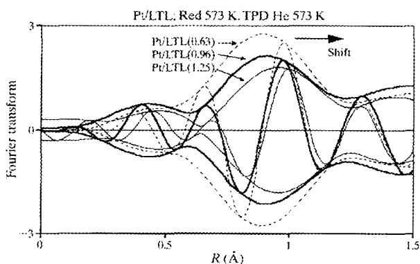
Figure 5 AXAFS spectra (FT, k^3 , \Delta k = 3 –13 \text{\AA}^{-1} ) of Pt/LTL catalysts after treatment in He.
