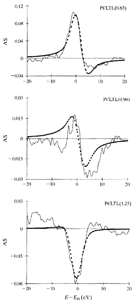
Figure 4 Results of analysis of near-edge spectra of H–Pt/LTL and Pt/LTL: Fano-resonance line shape ( i.e. AS) for Pt/LTL (solid line) and best fit to resonant line shape with parameters in Table 1.
