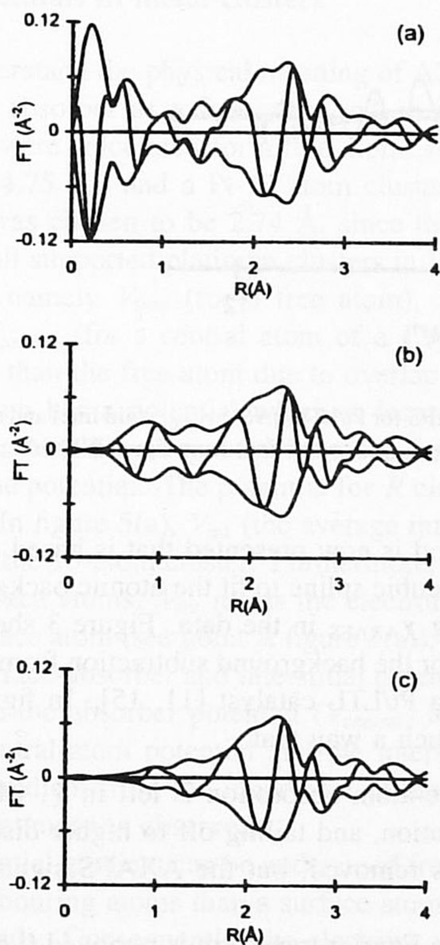
Figure 3. The Fourier transform ( k^1 \chi_{\text{total}} ; \Delta k : 3.0–13.5 Å -1 ) of experimental data from Pt/LTL (K/Al molar ratio = 0.96) after three different levels of background smoothing. (a) The free-atom signal is left in the data. (b) The free-atom scattering is removed, while the AXAFS signal is kept. (c) Background removal according to earlier criteria.
