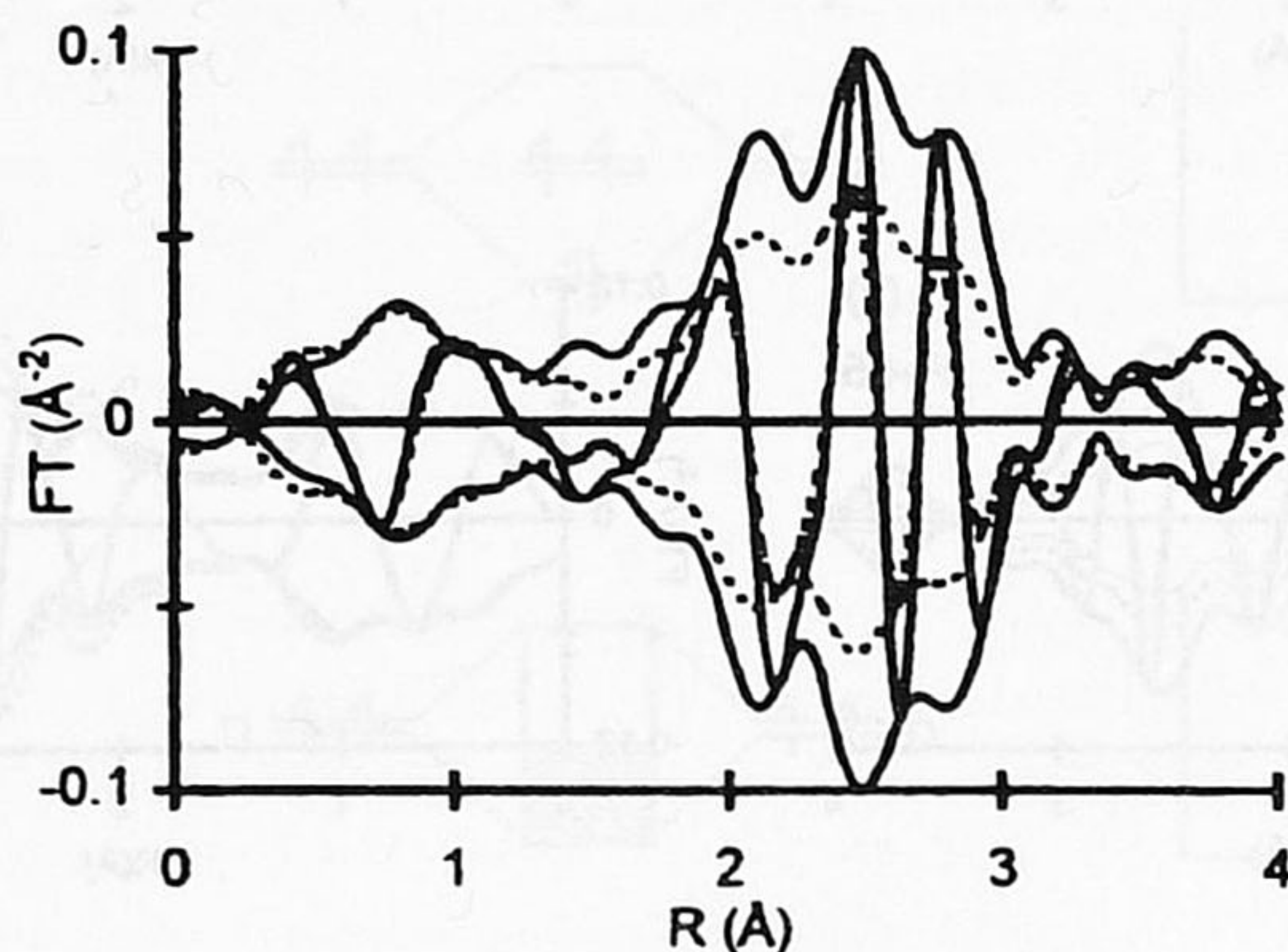
Figure 10. Comparison of Fourier transforms ( k^1 \chi_{\text{total}} ; \Delta k : 3–14 \text{\AA}^{-1} ) of experimental data for Pt clusters supported in Y zeolite catalysts with different average particle sizes: N_{\text{Pt-Pt}} (first shell) = 6 (solid line) and N_{\text{Pt-Pt}} (first shell) = 4.2 (dotted line).
