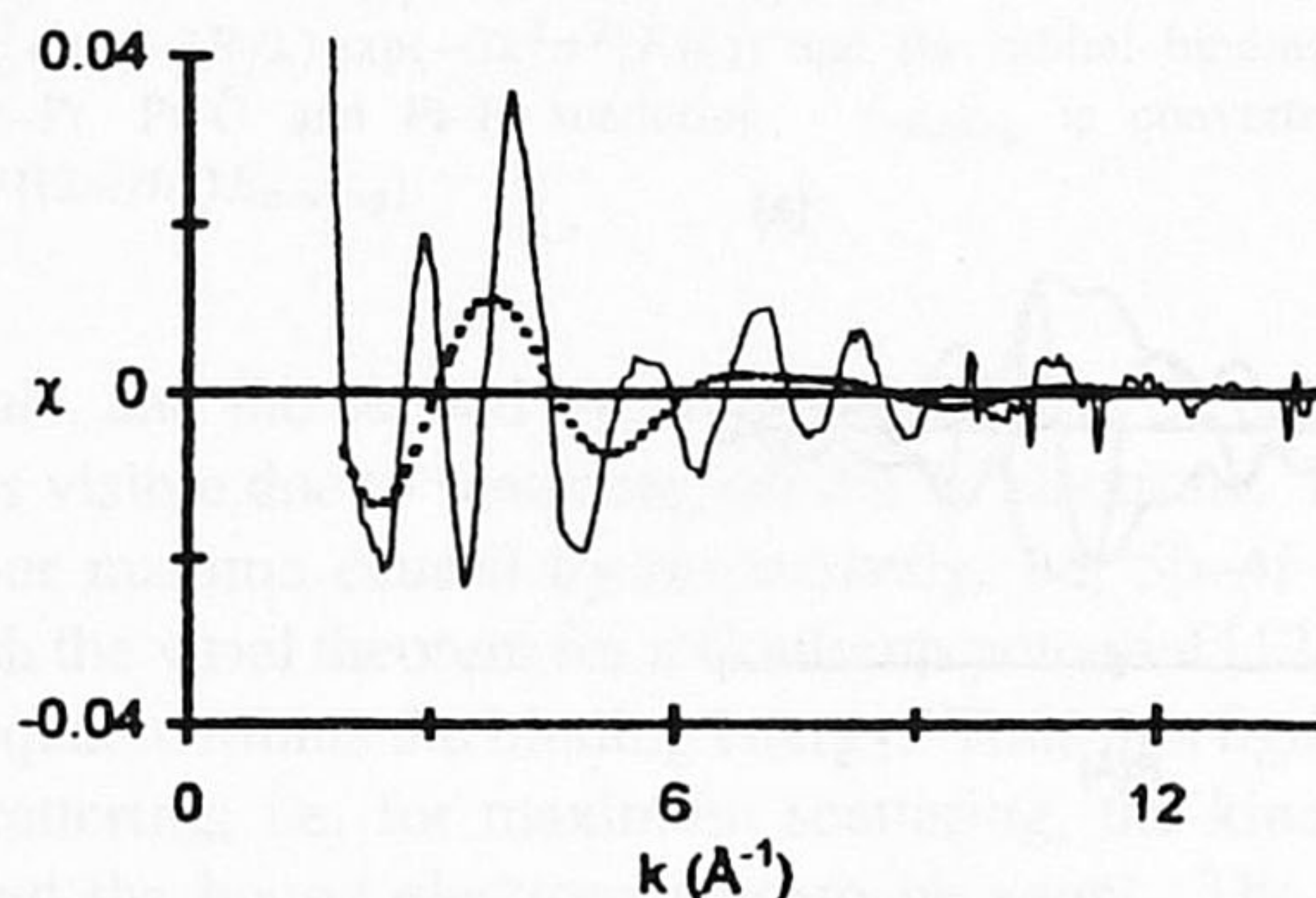
Figure 4. The experimental EXAFS for Pt/LTL(0.96) ( \chi_{\text{total}} , solid line) and the back-transformed Fourier-filtered AXAFS signal ( \chi_{\text{AXAFS}} , dotted line) from figure 3(b) ( \Delta k : 1.9–13.8 \text{\AA}^{-1} ; \Delta R : 0.14–1.58 \text{\AA} ).
