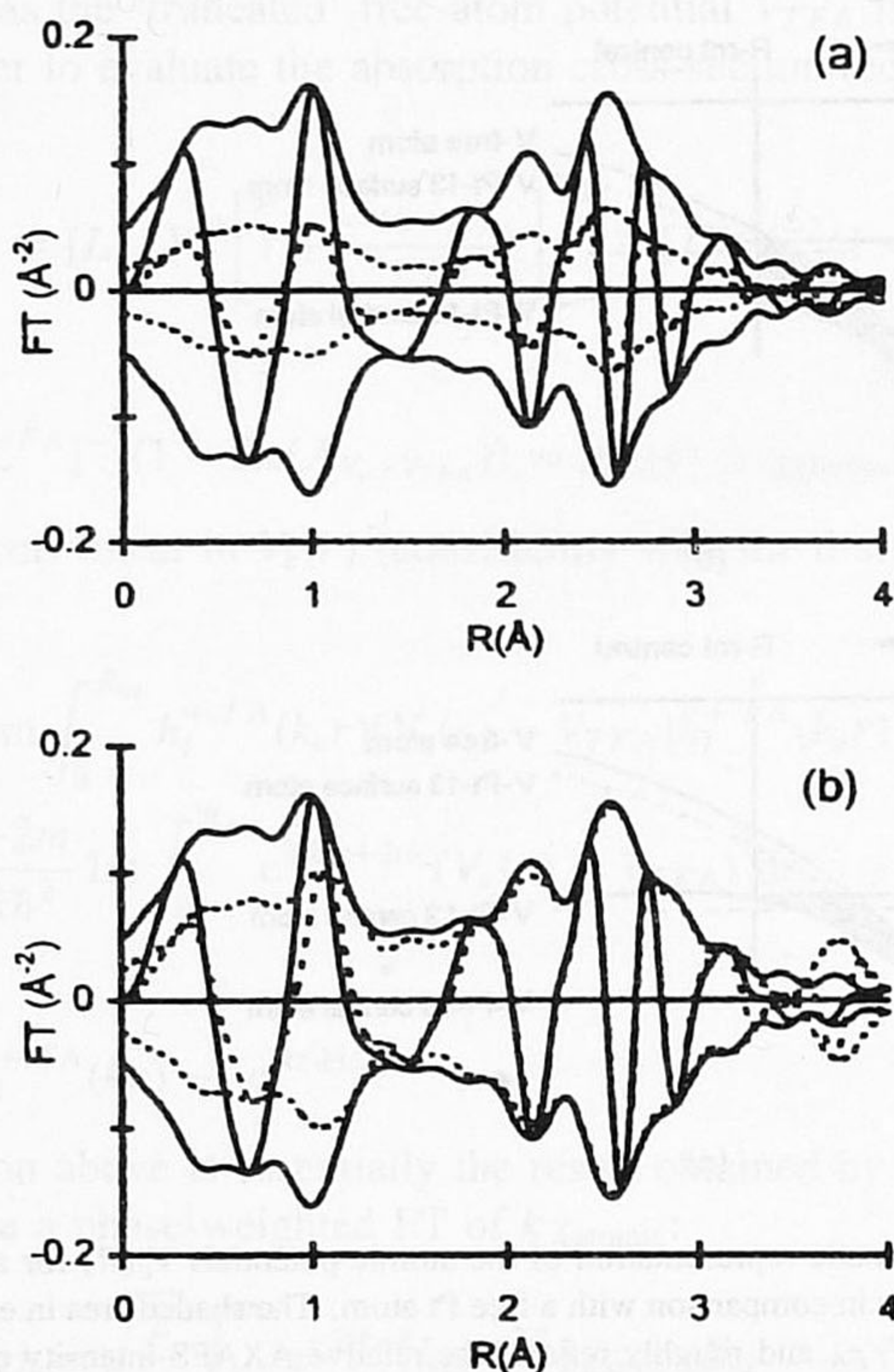
Figure 7. (a) Fourier transforms ( k^1 \chi_{\text{total}} ; \Delta k : 3–15 Å -1 ) of the FEFF7-calculated spectrum for a Pt-13 central atom (solid line) and a Pt-13 surface atom (dotted line). (b) Fourier transforms ( k^1 ; \Delta k : 3–15 Å -1 ) of the calculated \chi_{\text{total}} -spectrum for a Pt-13 central atom (solid line) and a Pt-55 central atom (dotted line).
