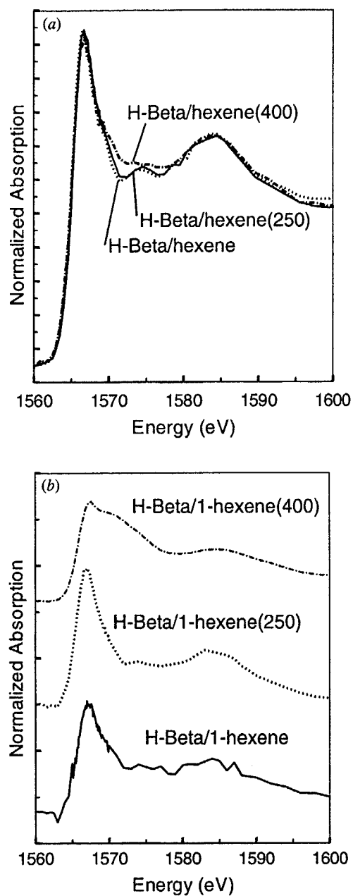
Figure 3. Fluorescence yield (a) and electron yield (b) detected spectra of H-Beta/1-hexene, H-Beta/1-hexene(250) and H-Beta/1-hexene(400). The latter spectrum differs from the other two by a surplus in intensity in the 3–7 eV range. The electron yield spectrum of H-Beta/1-hexene shows more noise, probably because this sample is less conductive than the others.
