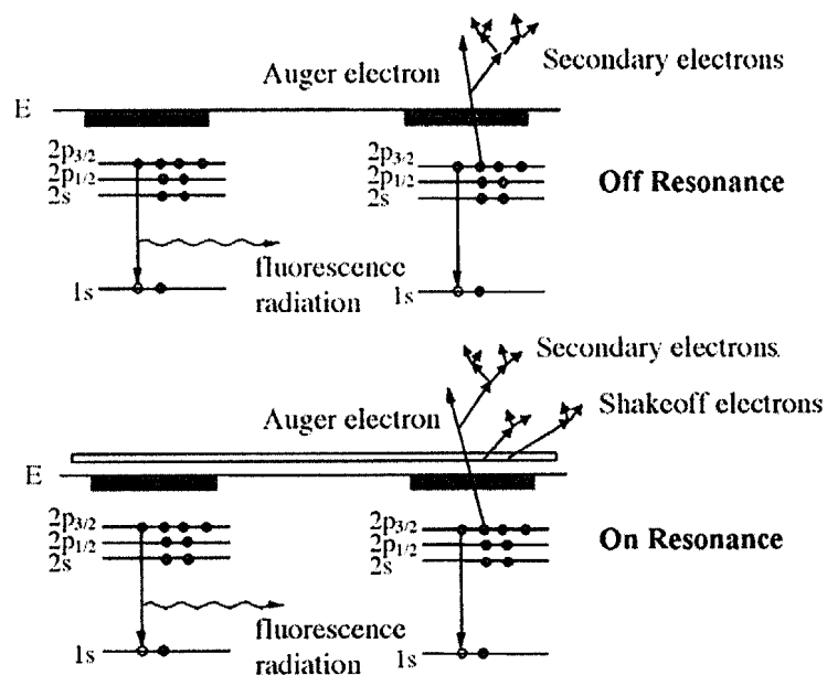
Figure 6. Schematic illustration of the dominant core hole decay processes off resonance (top) and on resonance (bottom) when CT from benzene to Al 3p has occurred. The KL_{23} (1s2p) fluorescence yield is the same for both on and off resonance, but the yield of secondary electrons is magnified on resonance because of the additional shake-off of the two electrons bound in the resonance. Conversely, the 'elastic' KL_{23}L_{23} (1s2p2p) Auger yield is diminished on resonance. (This figure is in colour only in the electronic version)
