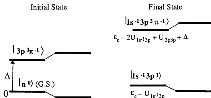
Figure 5. Energy diagram for the initial (ground) state and K-edge XAS final states in the correlated electron model (i.e. when U > \Gamma as discussed in the text). The energies are given for the initial state relative to the unmixed ground state |n^0\rangle (energy = 0), and the final state relative to the unmixed regular core hole excited state |1s^{-1}3p\rangle . The energy \Delta is the energy required to transfer an electron from the benzene \pi to the Al 3p (via the benzene \pi^* ). The parameters U_{1s^{-1}3p} and U_{3p3p} denote the corresponding Coulomb interaction energies. For both the initial and final states, the premixed state energies are given on the left, and mixed state energies on the right, illustrating the relatively small effects of covalent mixing compared to the correlation effects in this case.
