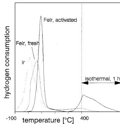
FIG. 2. Temperature programmed reduction profiles of Ir/SiO 2 and FeIr/SiO 2 catalysts. Pretreatment: reduction at 450°C and exposure to air at room temperature; activated catalyst: 48 h of reaction as in Fig. 1 followed by exposure to air at room temperature.
