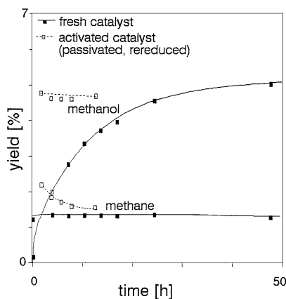
FIG. 1. Conversion of CO into methane and methanol (40 bar of 3H 2 + 1CO synthesis gas at 270°C). Comparison of the freshly reduced 1 : 1 FeIr/SiO 2 catalyst and the catalyst after 48 h of reaction, exposure to air at room temperature, and rereduction in H 2 at 400°C.
