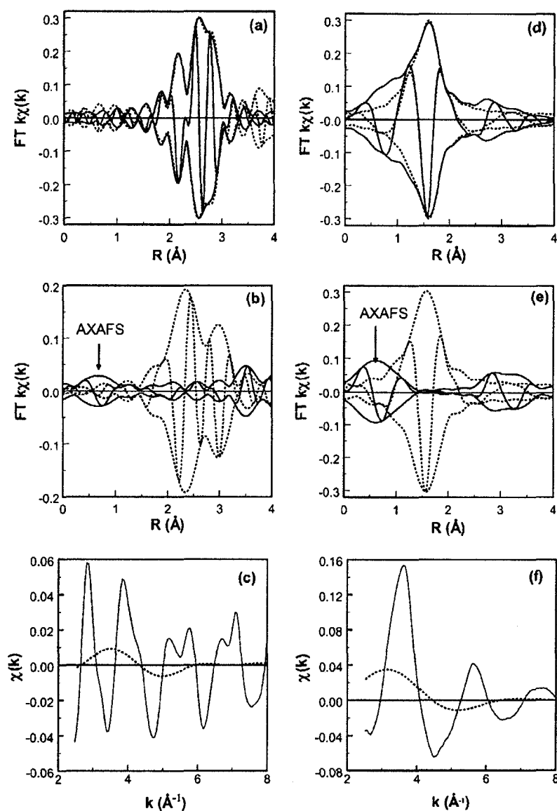
Figure 8. (a) FT ( k^1 , \Delta k = 2.5-15 \text{ \AA}^{-1} ) of the experimental XAFS (solid curve) and the first shell Pt-Pt fit (dotted curve) for Pt foil. (b) FT ( k^1 , \Delta k = 2.5-10 \text{ \AA}^{-1} ) of the first shell Pt-Pt fit (dashed curve) and the difference file (experimental XAFS minus first shell Pt-Pt fit) (solid curve) for Pt foil. (c) Isolated AXAFS (FT, k^1 , \Delta k = 2.5-10 \text{ \AA}^{-1} ; FT -1 , \Delta R = 0.2-1.7 \text{ \AA} ) (dotted curve) and experimental XAFS (solid curve). (d) FT ( k^1 , \Delta k = 2.5-13 \text{ \AA}^{-1} ) of the experimental XAFS (solid curve) and first shell Pt-O fit (dashed curve) for Na 2 Pt(OH) 6 . (e) FT ( k^1 , \Delta k = 2.5-10 \text{ \AA}^{-1} ) of the first shell Pt-O fit (dashed curve) and difference file (experimental XAFS minus first shell Pt-O fit) for Na 2 Pt(OH) 6 . (f) Isolated AXAFS (FT, k^1 , \Delta k = 2.5-10 \text{ \AA}^{-1} ; FT -1 , \Delta R = 0.3-1.5 \text{ \AA} ) (dotted curve) and experimental XAFS (solid curve).
