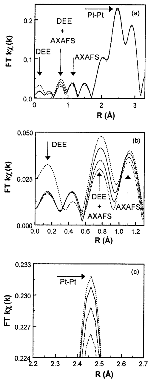
Figure 1. (a) FT ( k^1 , \Delta k = 1.5\text{--}12 \text{\AA}^{-1} ) of the Pt foil XAFS data for different characteristic values of the smooth parameter SM (dotted curve, 3.5; solid curve, 3.4; dashed curve, 3.3; dashed dotted curve, 3.2). The origin of the different peaks is indicated; DEE: double electron excitations, AXAFS: atomic XAFS, and Pt-Pt: first shell Pt-Pt peak. (b) Same as in (a) but with an expansion in the low R region. (c) Same as in (a) but with an expansion in the R region containing the first shell Pt-Pt peak.
