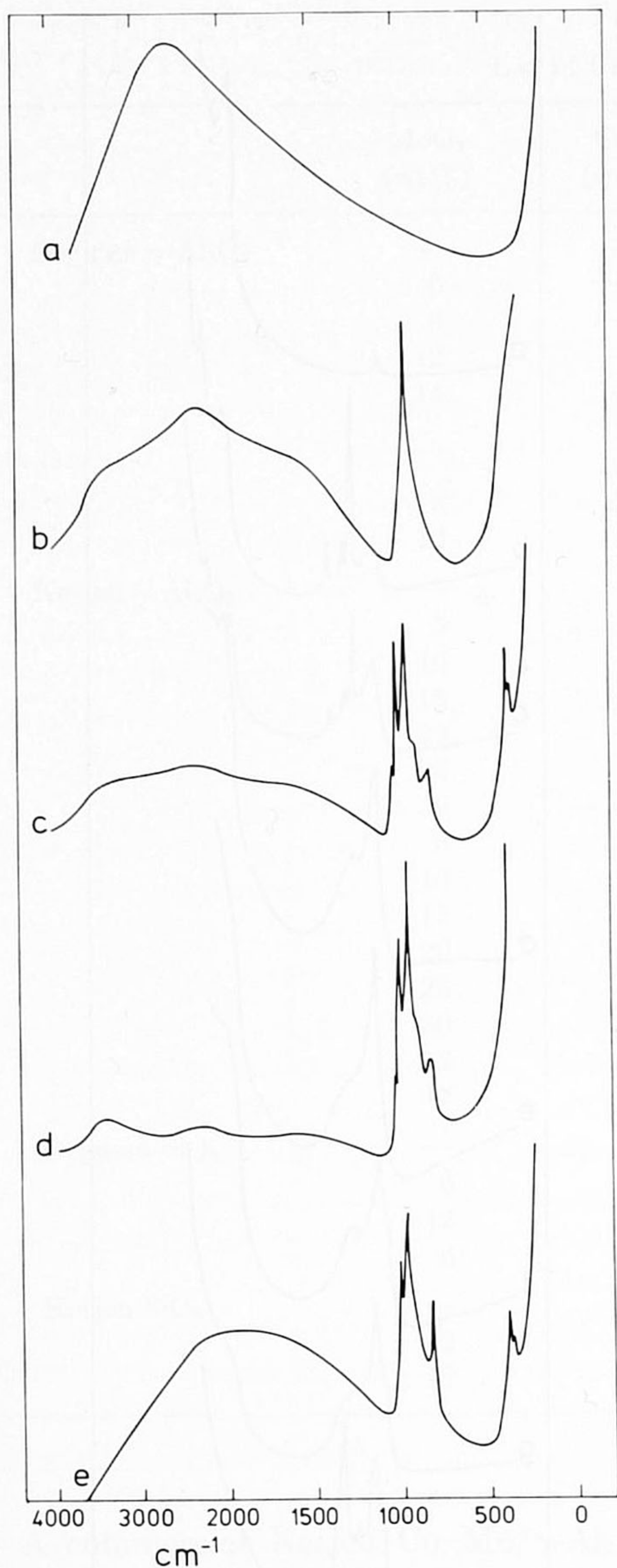
FIG. 2. Raman spectra of Mo/Al-D catalysts. (a) Carrier; (b) Mo(6)/Al-D; (c) Mo(9)/Al-K; (d) Mo(12)/Al-D; (e) Mo(15)/Al-D.
