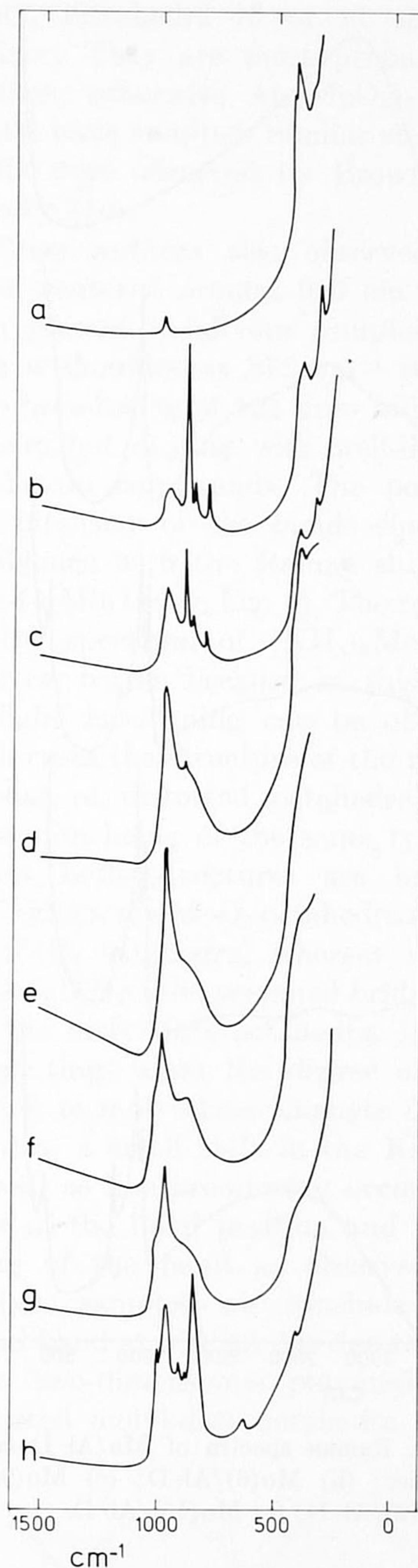
FIG. 1. Raman spectra of Mo/Al-K catalysts. (a) Carrier; (b) Mo(5)/Al-K; (c) Mo(10)/Al-K; (d) Mo(15)/Al-K; (e) Mo(20)/Al-K; (f) Mo(25)/Al-K; (g) Mo(30)/Al-K; (h) Mo(30)/Al-K. All samples except h were treated for 16 h in oxygen at 873 K. Due to fluorescence and variations in the positioning of the samples, intensities are not proportional to Mo content.
