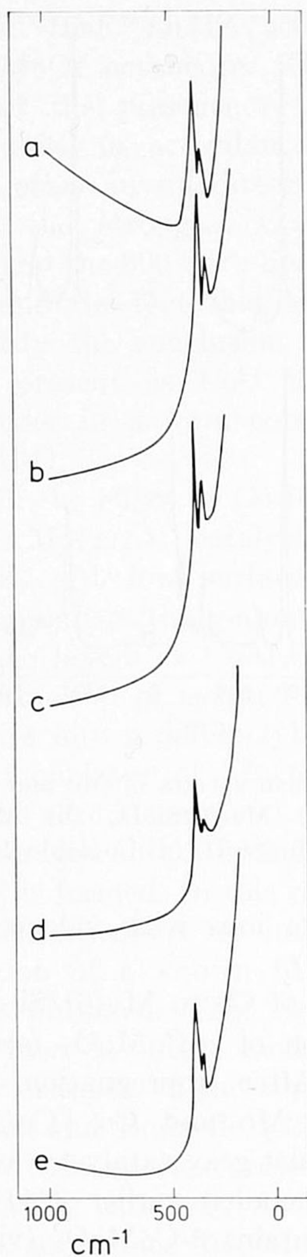
FIG. 9. Raman spectra of sulfided catalysts. (a) Mo(12)/Al-K; (b) Co(4)Mo(12)/Al-K; (c) Mo(12)/Si-K; (d) Co(4)Mo(12)/Si-K; (e) MoS 2 (10)/Al-K.
