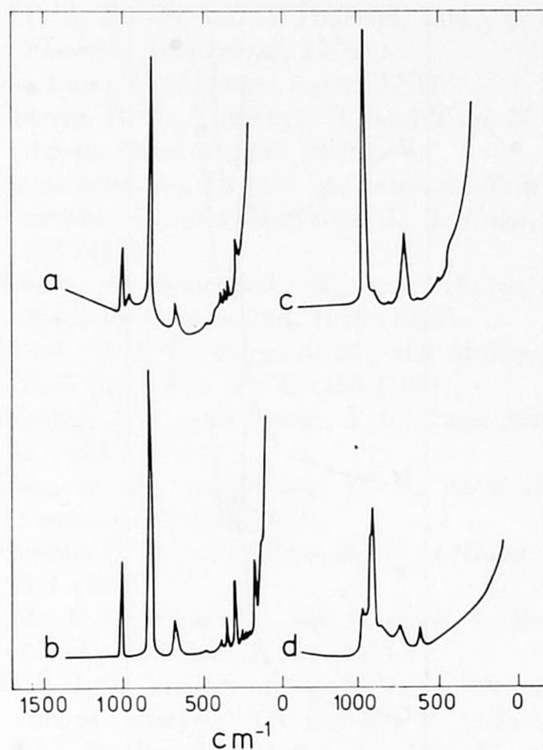
FIG. 8. Raman spectra of Mo and Co on silica catalysts. (a) Mo(6)/Si-D; (b) Mo(12)/Si-D; (c) Co(2)Mo(6)/Si-D; (d) Co(4)Mo(12)/Si-K.
