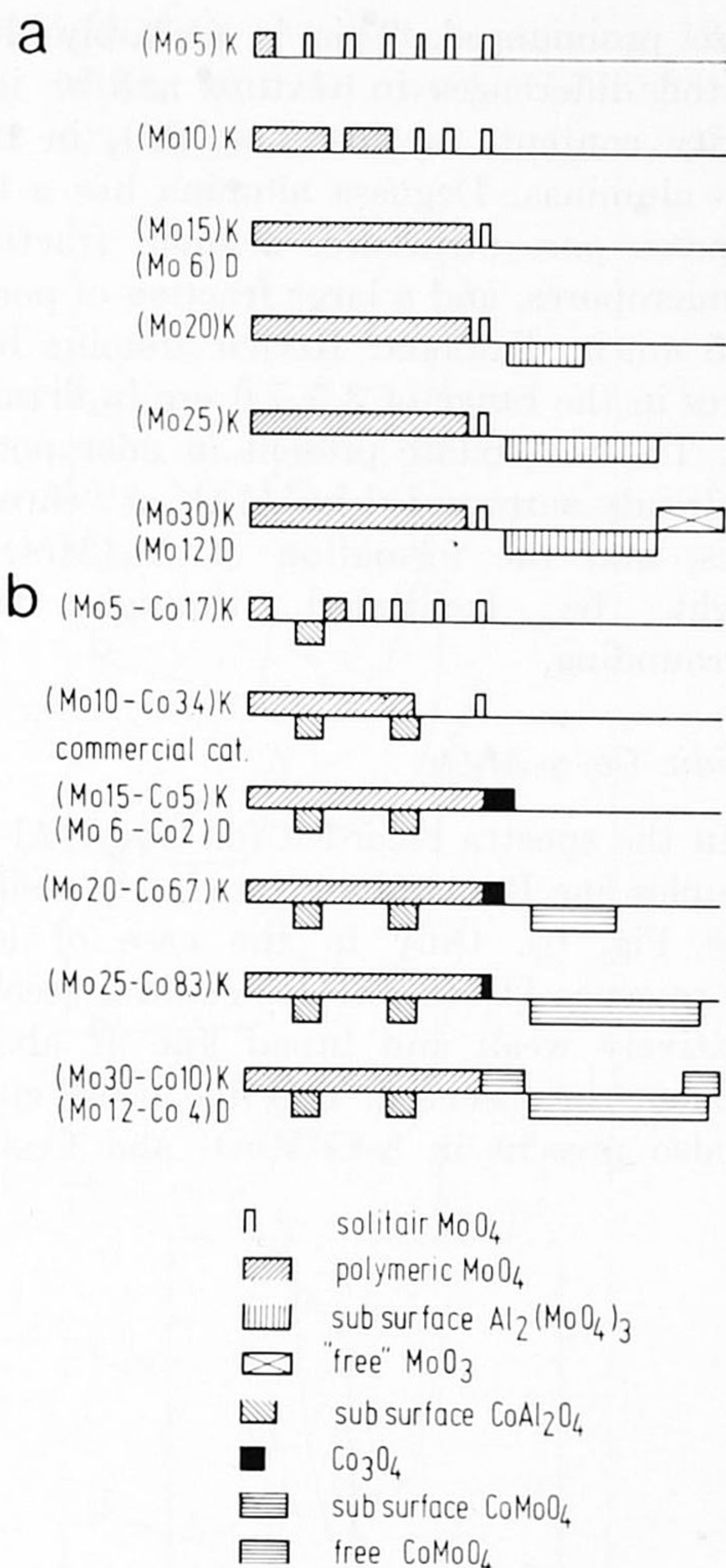
FIG. 5. (a) Upper six diagrams: coverage of the surface of alumina with the different molybdenum species, depending on the degree of surface coverage. (b) Lower six diagrams: coverage of the surface of alumina with the different molybdenum and cobalt species, depending on the degree of surface coverage.
