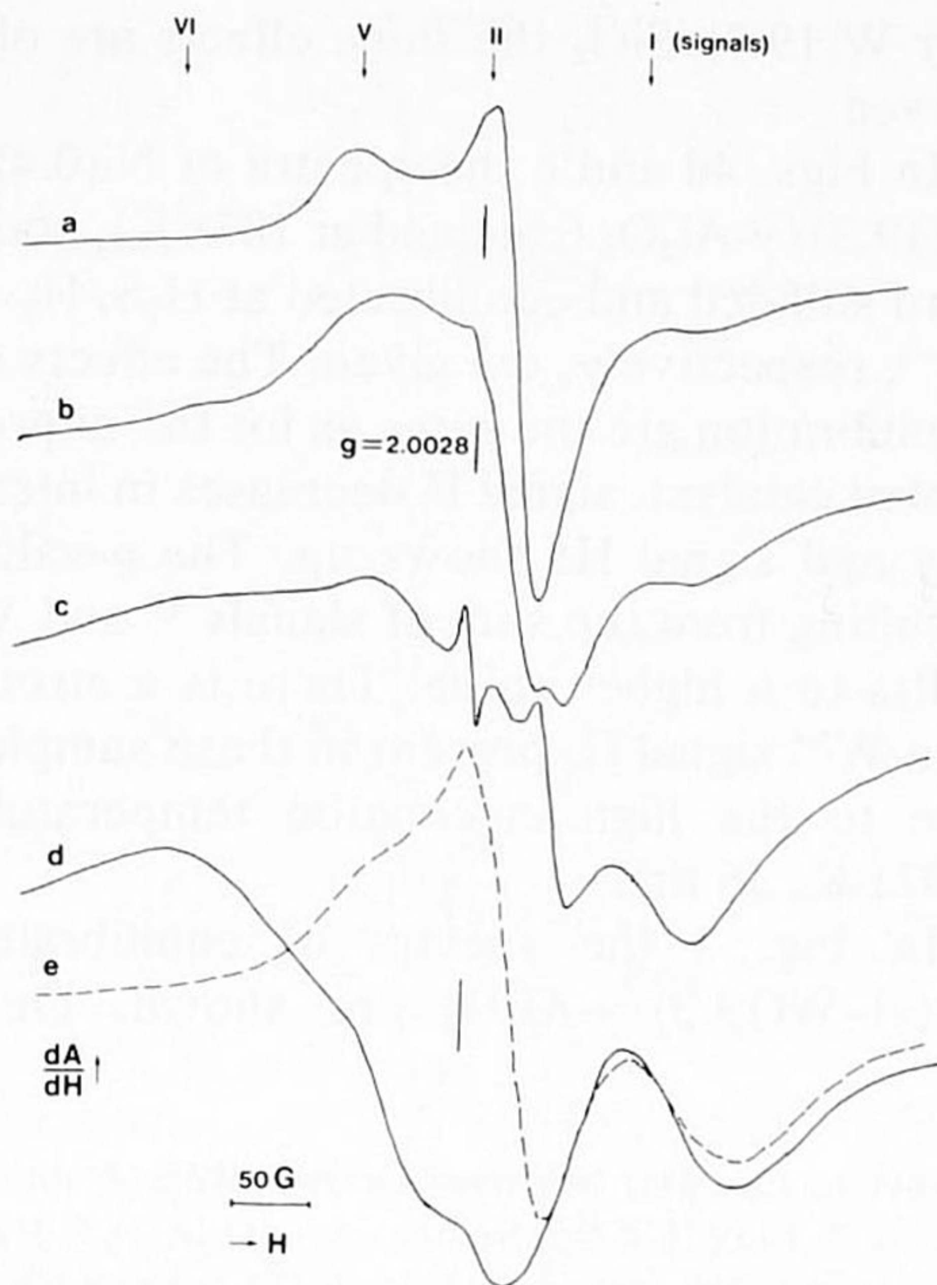
FIG. 1. ESR spectra (recorded at 20 K): (a) Mo(12)/SiO 2 , receiver gain (RG) 10 2 ; (b) Ni(0.4)-Mo(12)/SiO 2 , RG 2 × 10 2 ; (c) Ni(4)-Mo(12)/SiO 2 , RG 5 × 10 2 ; (d) Ni(4)-Mo(12)/γ-Al 2 O 3 , RG 5 × 10 2 ; (e) Mo(12)/γ-Al 2 O 3 , RG 10 2 . All samples are standard sulfided, for details see Experimental section. Numbers in parentheses are wt% NiO and MoO 3 , respectively.
