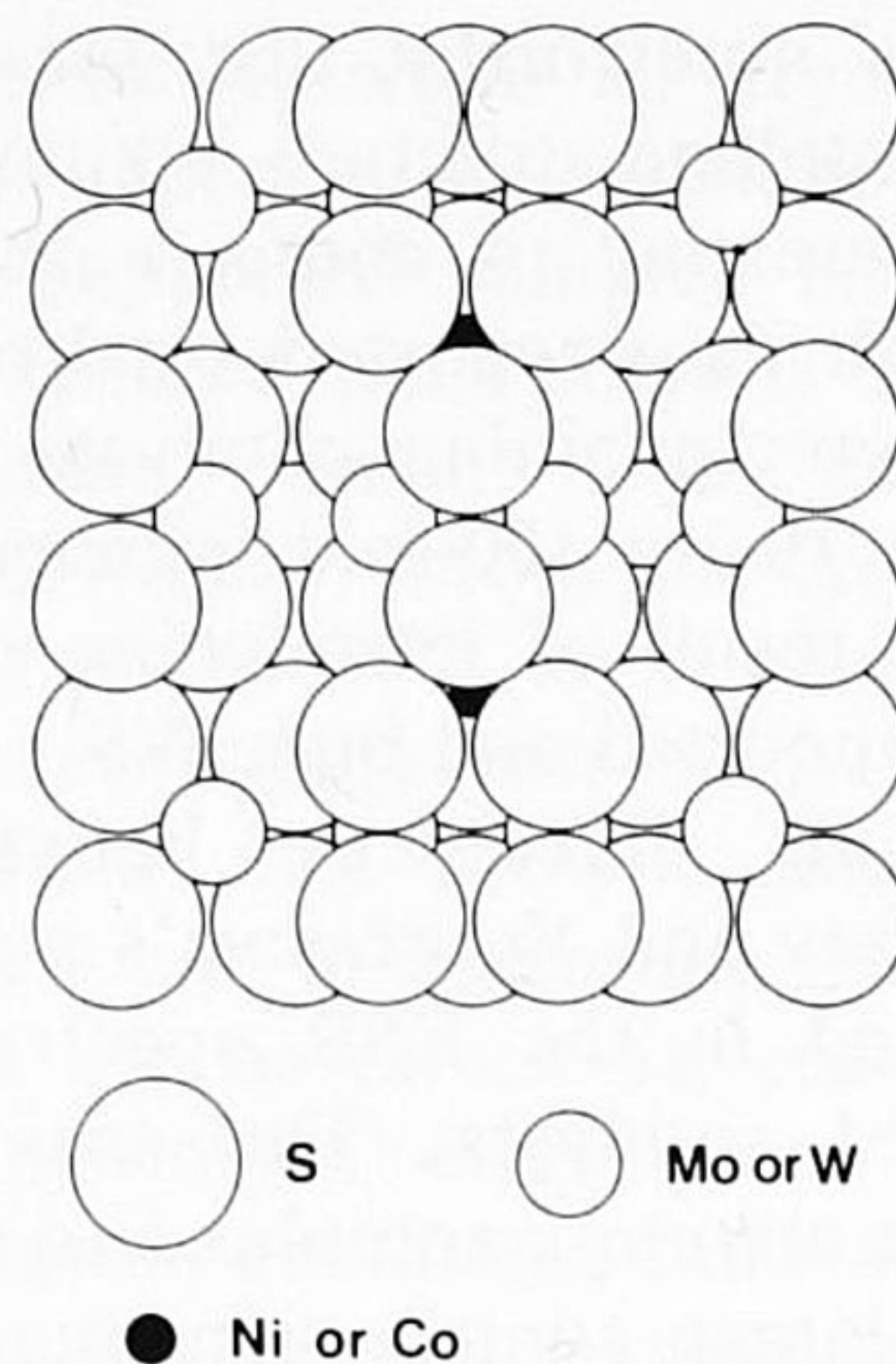
FIG. 9 \{10\bar{1}0\} surface of WS_2 ( MoS_2 ), with ideal ordered surface sulfur due to decoration by Ni or Co.
