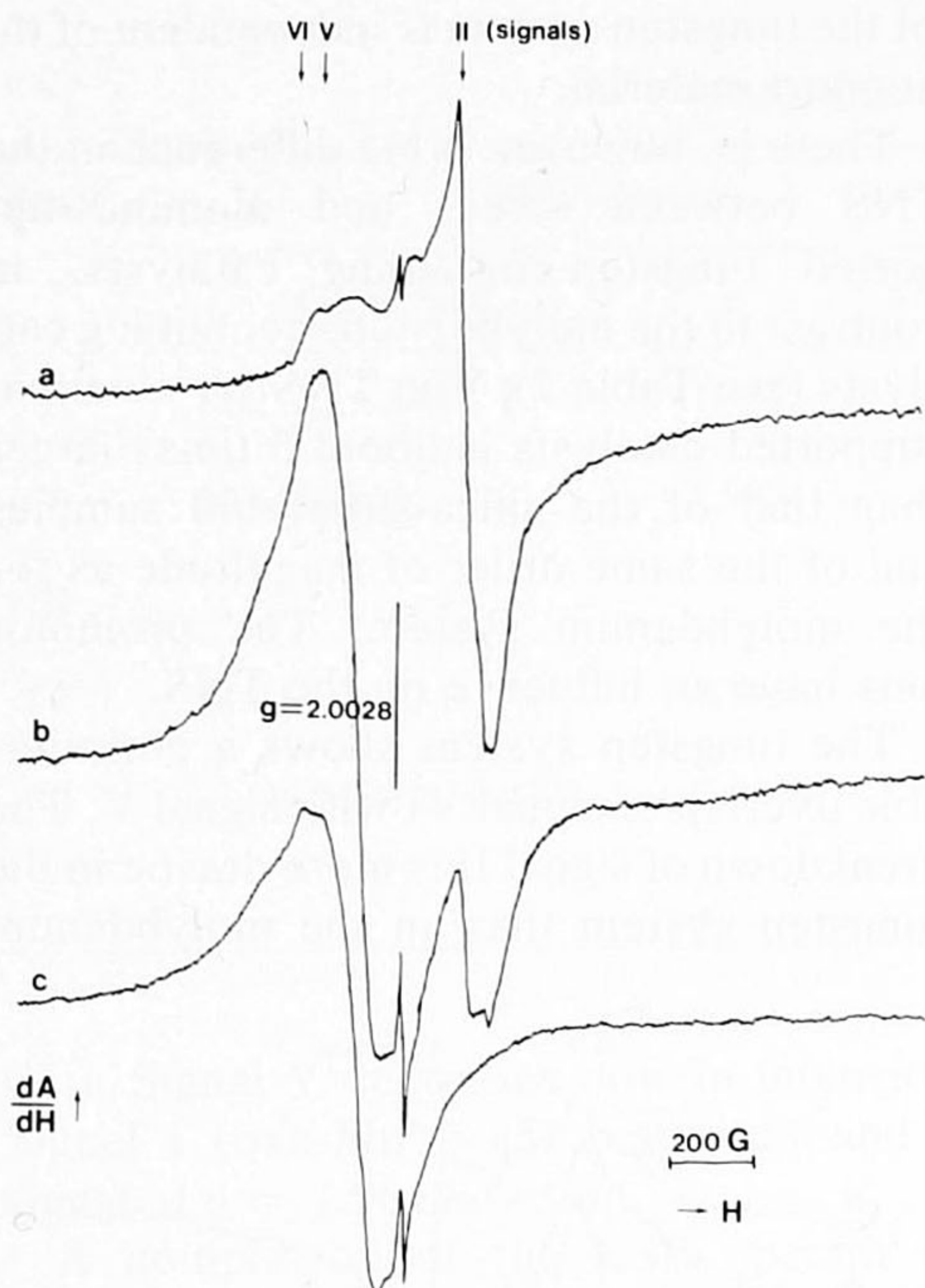
FIG. 3. ESR spectra (recorded at 20 K): (a) W(19.3)/ \gamma -Al 2 O 3 , RG 10 3 ; (b) Ni(0.4)-W(19.3)/ \gamma -Al 2 O 3 , RG 10 3 ; (c) Ni(4)-W(19.3)/ \gamma -Al 2 O 3 , RG 5 × 10 2 . All samples are standard sulfided.
