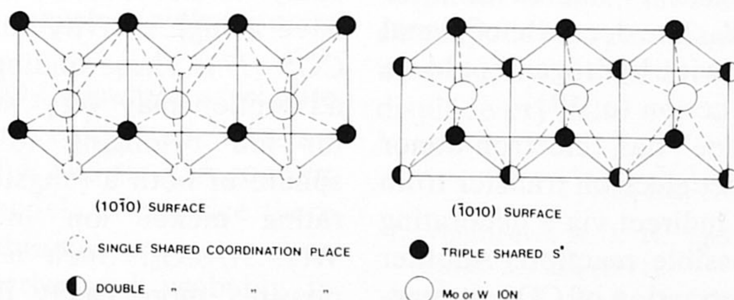
FIG. 8. Edge structure of \text{WS}_2 ( \text{MoS}_2 ) crystals.
