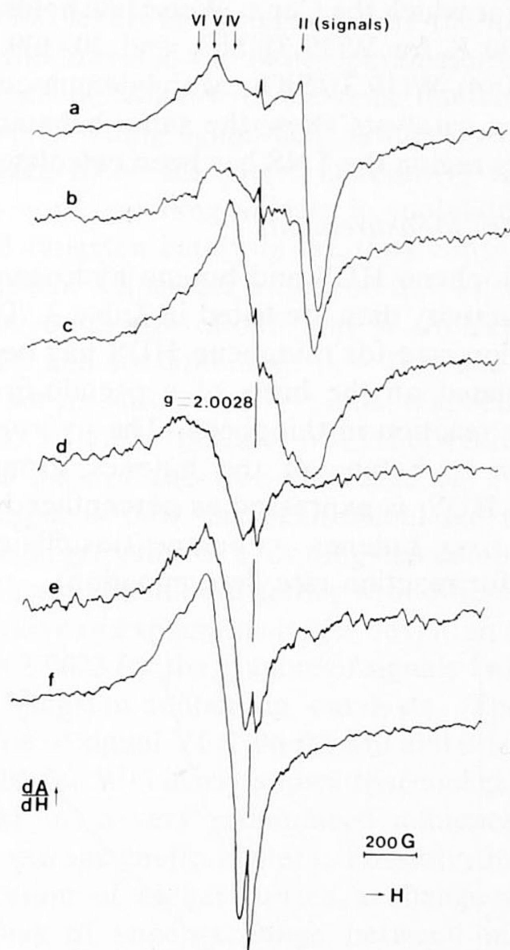
FIG. 6. ESR spectra (recorded at 20 K): (a) W(19.3)/SiO 2 , standard sulfided, evacuated at 295 K, RG 5 \times 10^3 ; (b) W(19.3)/SiO 2 , standard sulfided + 40 Torr CO at 295 K, RG 5 \times 10^3 ; (c) W(19.3)/SiO 2 , standard sulfided + 40 Torr CO at 473 K, RG 5 \times 10^3 ; (d) Ni(4)-W(19.3)/SiO 2 , standard sulfided, RG 2 \times 10^3 ; (e) Ni(4)-W(19.3)/SiO 2 , standard sulfided + 40 Torr CO at 295 K, RG 2 \times 10^3 ; (f) Ni(4)-W(19.3)/SiO 2 , standard sulfided + 40 Torr CO at 473 K, RG 10^3 . For details about CO adsorption procedure see Experimental section.
