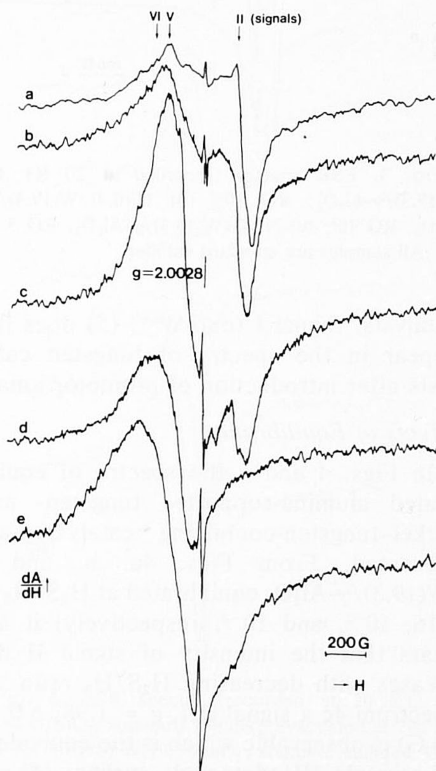
FIG. 2. ESR spectra (recorded at 20 K): (a) W(19.3)/SiO 2 , RG 5 × 10 3 ; (b) Co(0.4)-W(19.3)/SiO 2 , RG 4 × 10 3 ; (c) Ni(0.4)-W(19.3)/SiO 2 , RG 4 × 10 3 ; (d) Ni(4)-W(19.3)/SiO 2 , RG 4 × 10 3 ; (e) Co(4)-W(19.3)/SiO 2 , RG 8 × 10 3 . All samples are standard sulfided. Numbers in parentheses are wt% NiO, CoO, and WO 3 , respectively.
