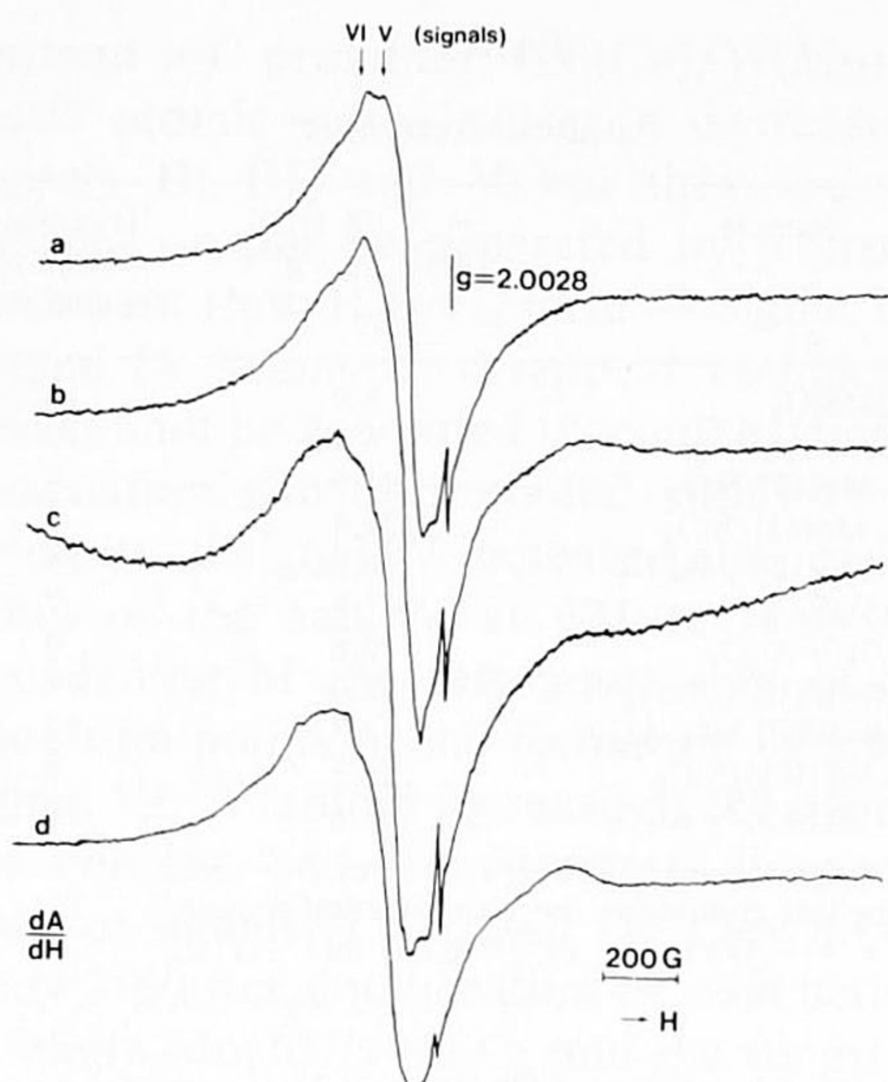
FIG. 5. ESR spectra (recorded at 20 K) of Ni(4)-W(19.3)/ \gamma -Al 2 O 3 : (a) standard sulfided, RG 5 \times 10^2 ; (b) equilibrated at 673 K, H 2 S/H 2 = 10^{-2} , RG 5 \times 10^2 ; (c) equilibrated at 673 K, H 2 S/H 2 = 10^{-4} , RG 10^3 ; (d) equilibrated at 613 K, H 2 S/H 2 = 10^{-4} , RG 5 \times 10^2 .
