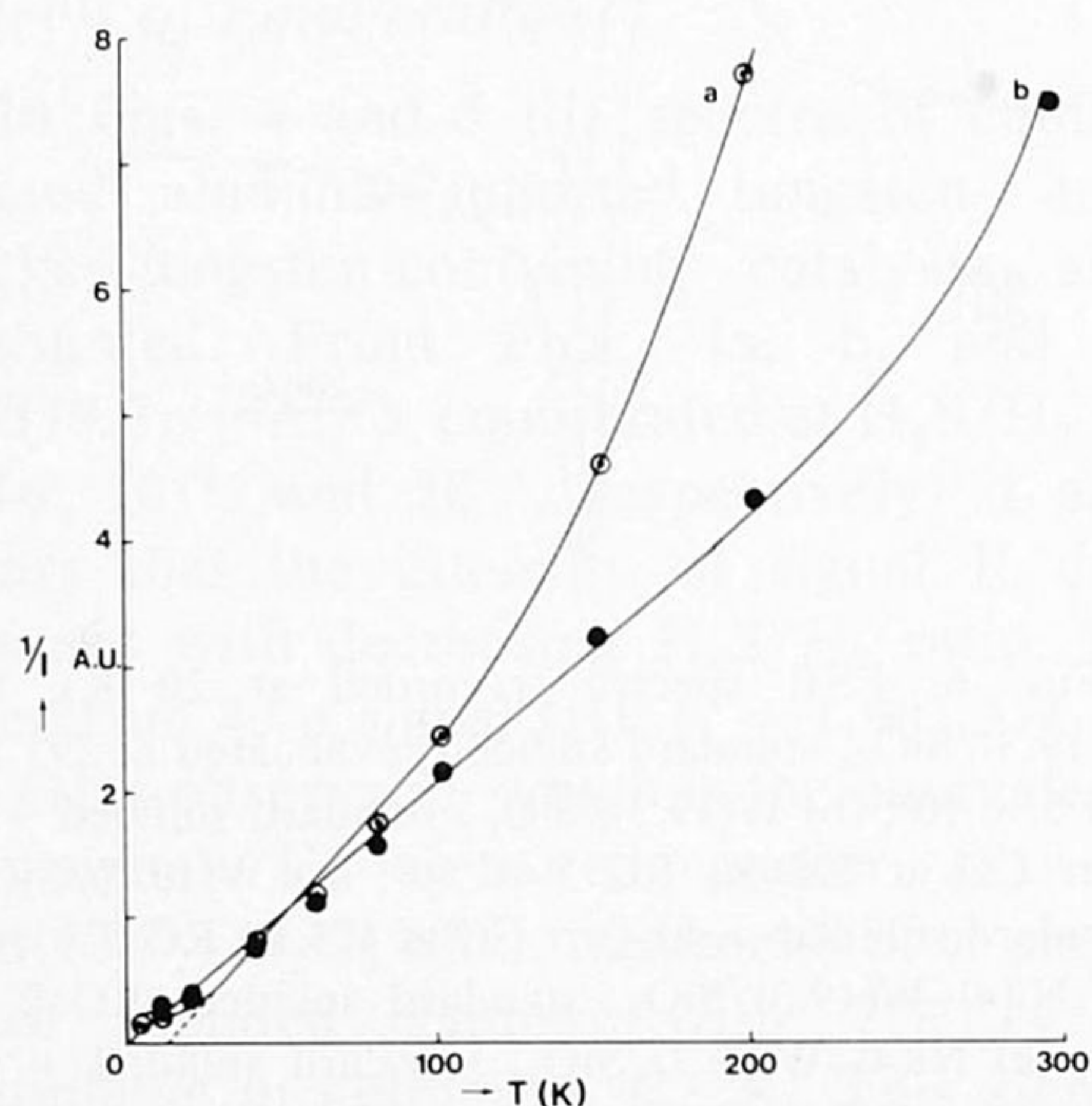
FIG. 7. Temperature dependence of the signal (II–VI) intensity. (a) Ni(4)-W(19.3)/SiO 2 ; (b) W(19.3)/SiO 2 . Standard sulfided samples.
