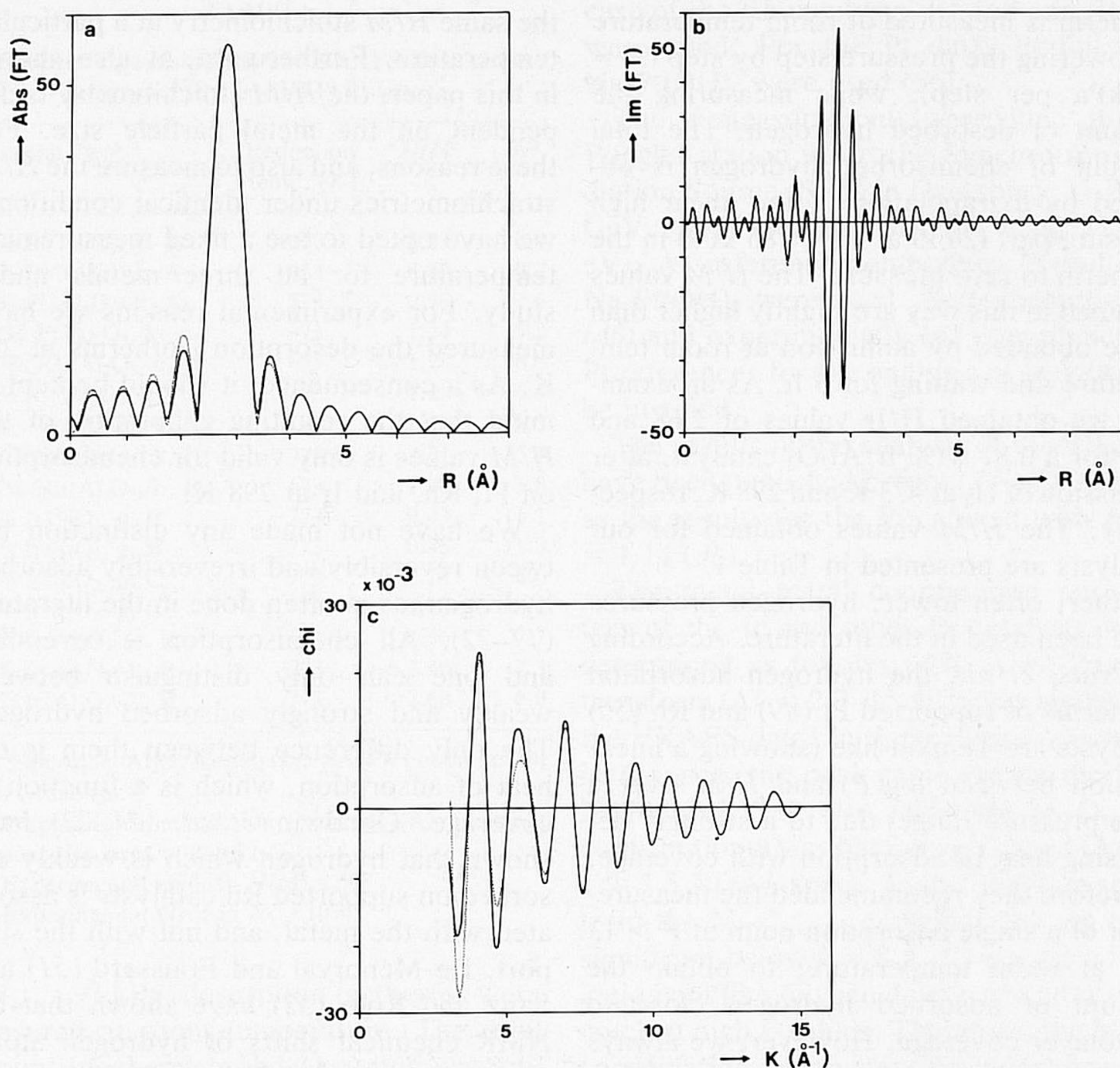
FIG. 1. Fit obtained in the EXAFS analysis of 4.2 wt% Pt/Al 2 O 3 , H/Pt = 0.77; (—) experiment, (···) fit. (a) Amplitude of the Fourier transform of the EXAFS obtained by a k^3 Fourier transform between k = 7.9 and 13.8 \text{ \AA}^{-1} ; (b) imaginary part of the Fourier transform; (c) fit in k -space. The Pt–Pt spectrum has been calculated on the basis of the fit for 7.9 < k < 13.8 \text{ \AA}^{-1} , with N = 7.6 , R = 2.75 \text{ \AA} , and \Delta\sigma^2 = 0.0035 \text{ \AA}^2 .
