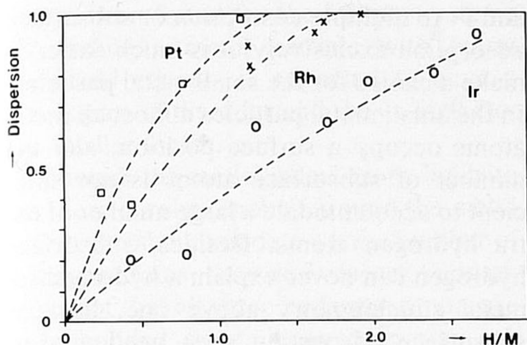
FIG. 4. Dispersion ( M_{\text{surface}}/M_{\text{total}} ) obtained on the basis of model calculations ( \alpha = 0.5 ) for Pt (□), Rh (×), and Ir (○), versus H/M .
