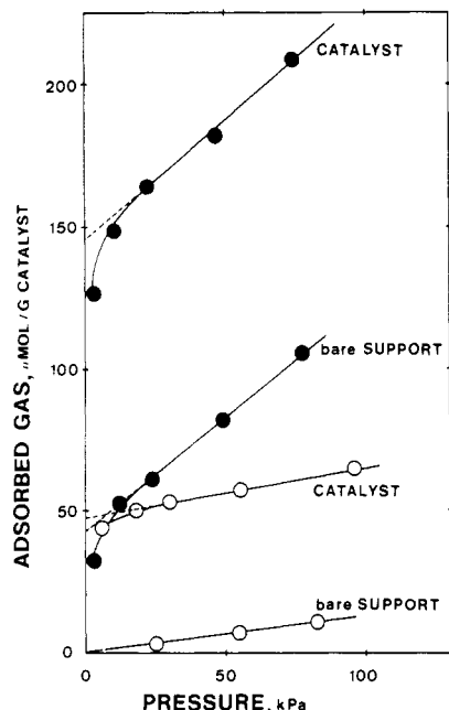
Figure 1. H 2 (○) and CO (●) chemisorption isotherms (measured at 298 K).
