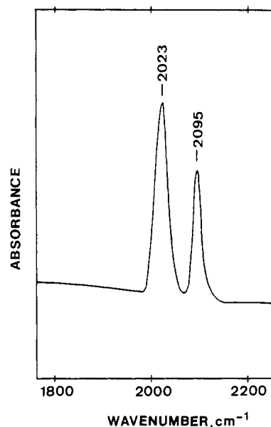
Figure 2. CO infrared spectrum on a 0.57 wt % Rh/γ-Al 2 O 3 (measured at 298 K).
