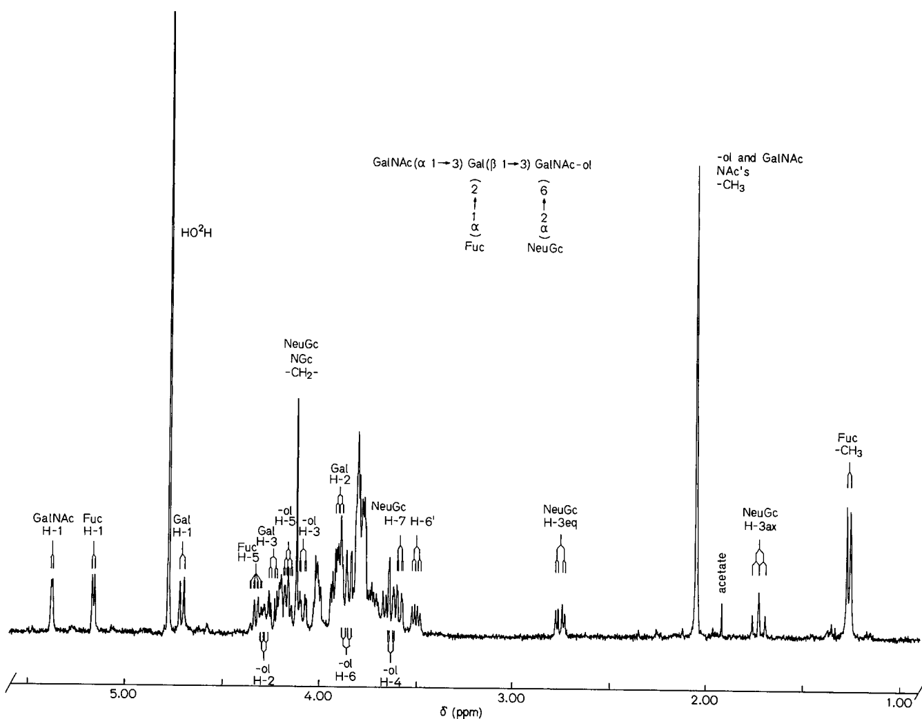
Fig. 2. 360-MHz 1 H-NMR spectrum of the acidic pentasaccharide-alditol in 2 H 2 O at 25°C
