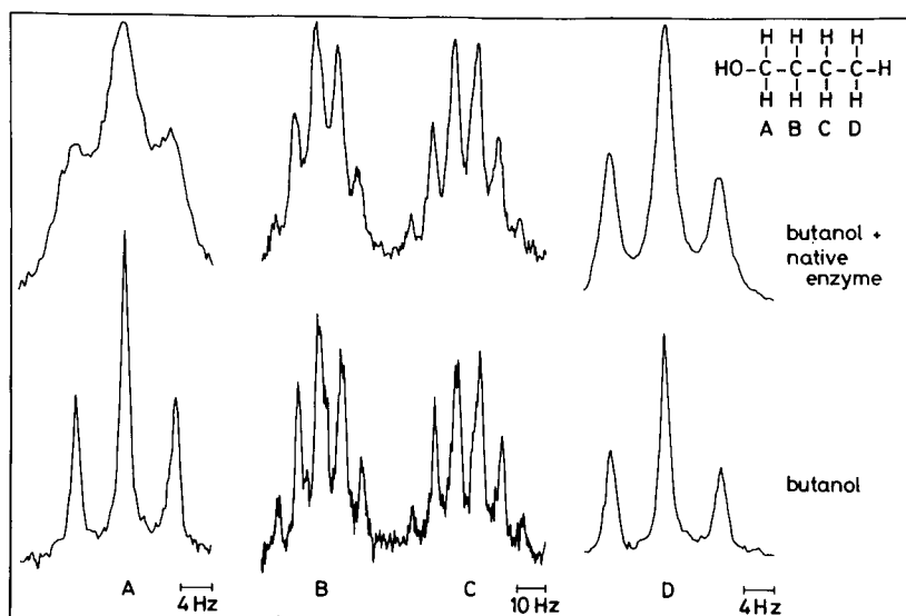
Fig. 2. NMR spectra of butanol-1 showing the effect of paramagnetic iron in native lipoxigenase-1 on the proton resonances of butanol-1. Lower spectrum: 8 mM butanol-1. Upper spectrum: 27 \mu l native lipoxigenase (0.52 mM) was added to 500 \mu l butanol-1 (24 mM). Final concentrations: lipoxigenase 26.6 \mu M and butanol-1 22.8 mM in 0.1 M borate buffer/D 2 O pH 9.0. Temperature 297 K.
