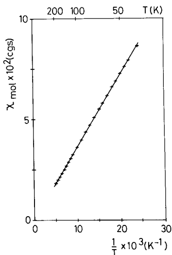
Fig. 1. The temperature dependent contribution of the magnetic susceptibility of native lipooxygenase-1, 103 \mu l 1.19 mM in 0.1 M boric acid/NaOH buffer pH 9.0.
