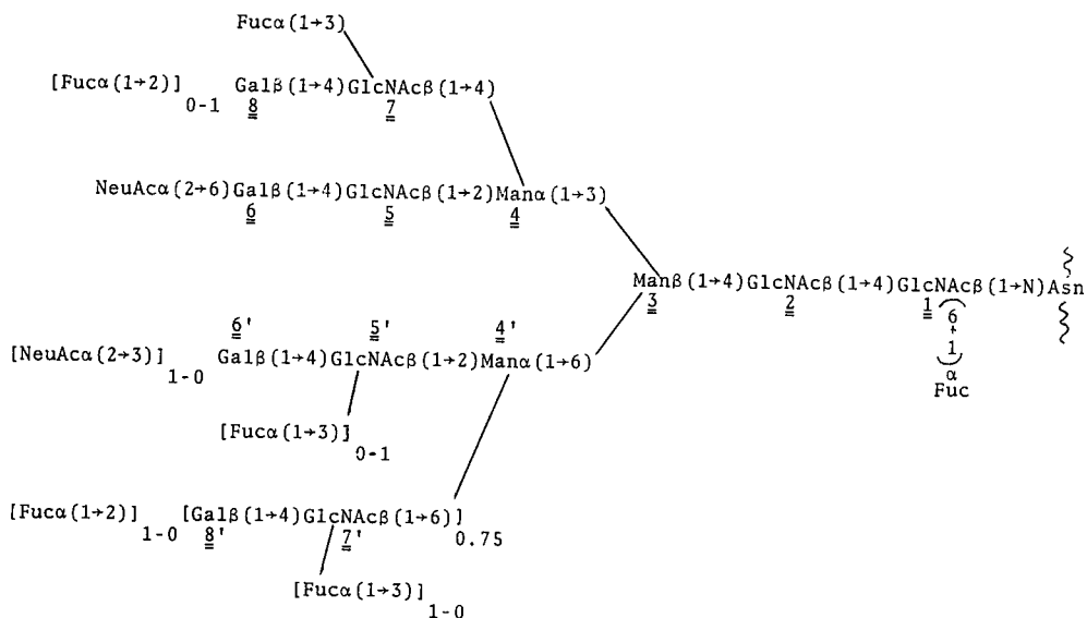
Fig. 2. The structures of the N-glycosidic tri- and tetra-antennary carbohydrate chains of human \gamma -seminoprotein. Note, the tri-antennary structure lacks the \underline{8}' - \underline{7}' branch and accounts for 25% of the mixture of these carbohydrate chains.
