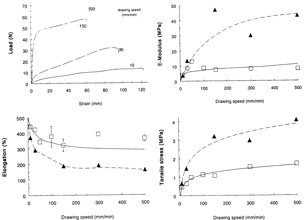
Figure 4 Load diagrams (upper left, 13–14% water) at different drawing speeds of amorphous TPS materials. Influence of drawing speed on the mechanical properties of amorphous TPS for two water contents (upper right and bottom): (□) 14–15% water, (▲) 13–14% water.
