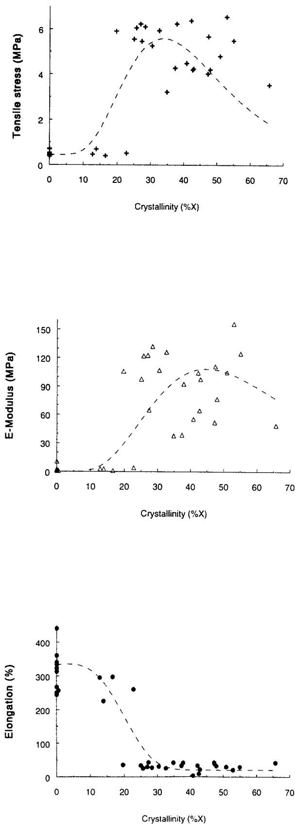
Figure 8 Influence degree of crystallization on the stress-strain properties of the waxy maize TPS materials at a water content of 13–15%.
