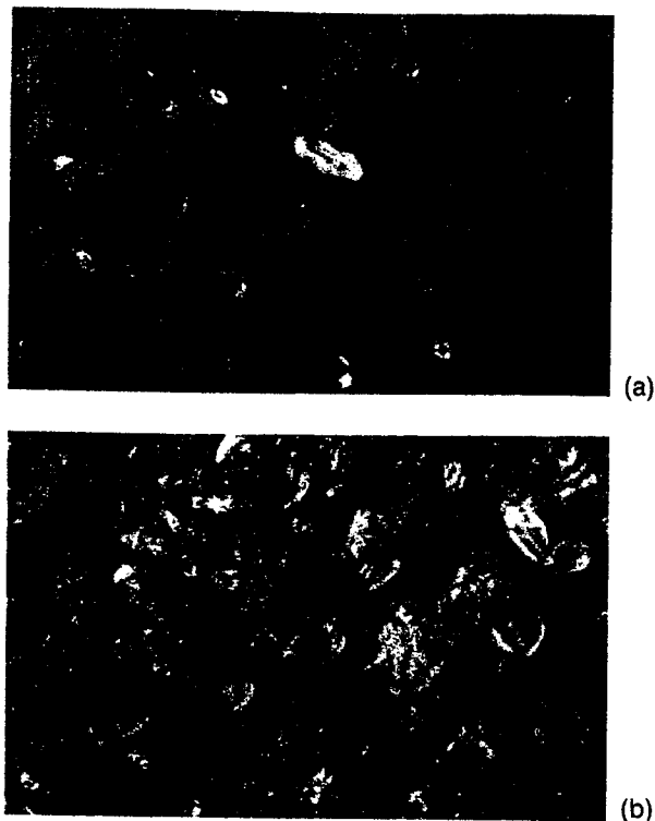
Figure 1 Polarized light microscopy of waxy maize starch TPS materials (batch WCN1) (a, 9.6% water) directly and (b, 13% water) after storage at 60% RH.
