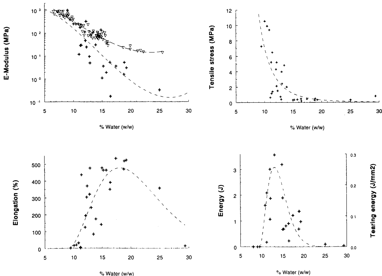
Figure 3 Mechanical properties of amorphous waxy maize TPS materials (batch WCN1) as a function of water content: (+) waxy corn starch, (∇) potato starch.
