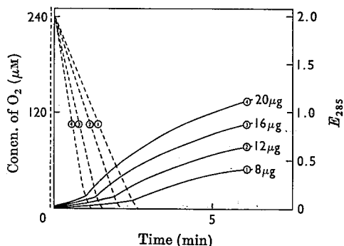
Fig. 2. Progress curves for the lipoxygenase-induced reaction of linoleic acid followed spectrophotometrically at 285 nm (—) and by simultaneous polarographic determination of the O 2 concentration (---). To the substrate solution (saturated with air at 25°C and containing 240 μM-O 2 ) was added the indicated amount of enzyme (8-20 μg) dissolved in 10 μl of buffer.
