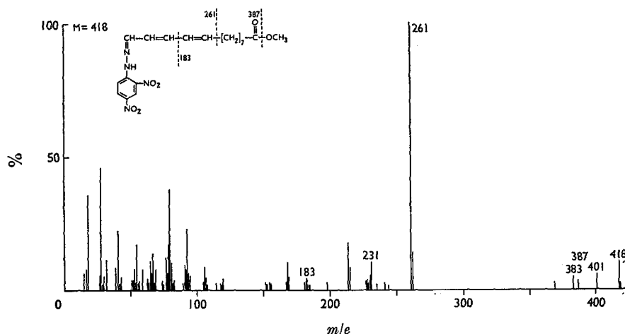
Fig. 1. Mass spectrum of the DNP-hydrazone of methyl 13-oxotrideca-9,11-dienoate.
