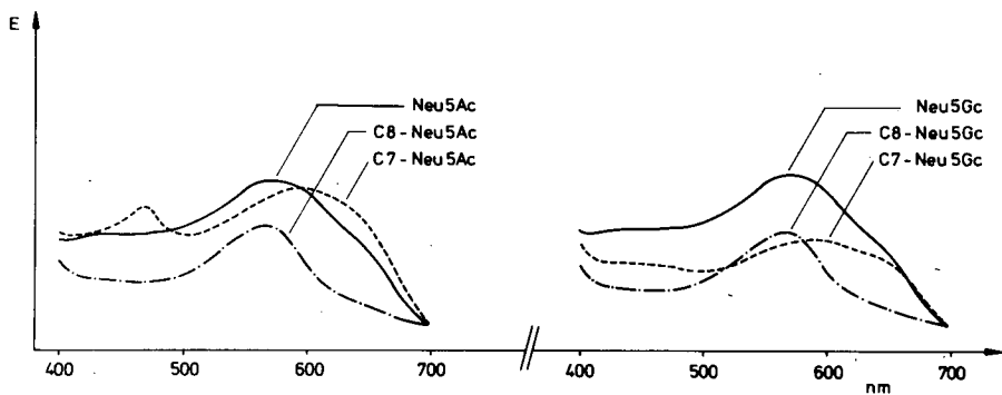
Figure 2. Absorption curves of the chromophores obtained from Neu5Ac or Neu5Gc and their C-7/C-8 analogues in the orcinol/Fe 3+ /HCl assay between 400 and 700 nm.
