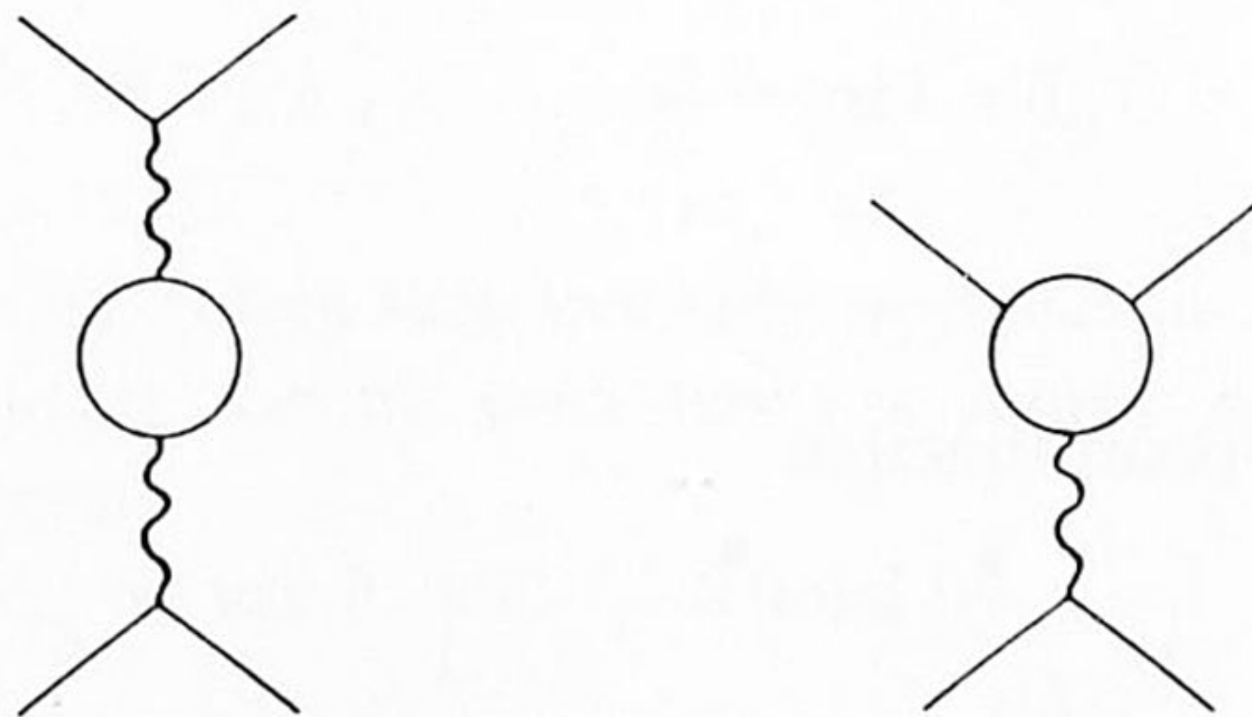
Fig. 2. Non-vanishing diagrams for large m .
