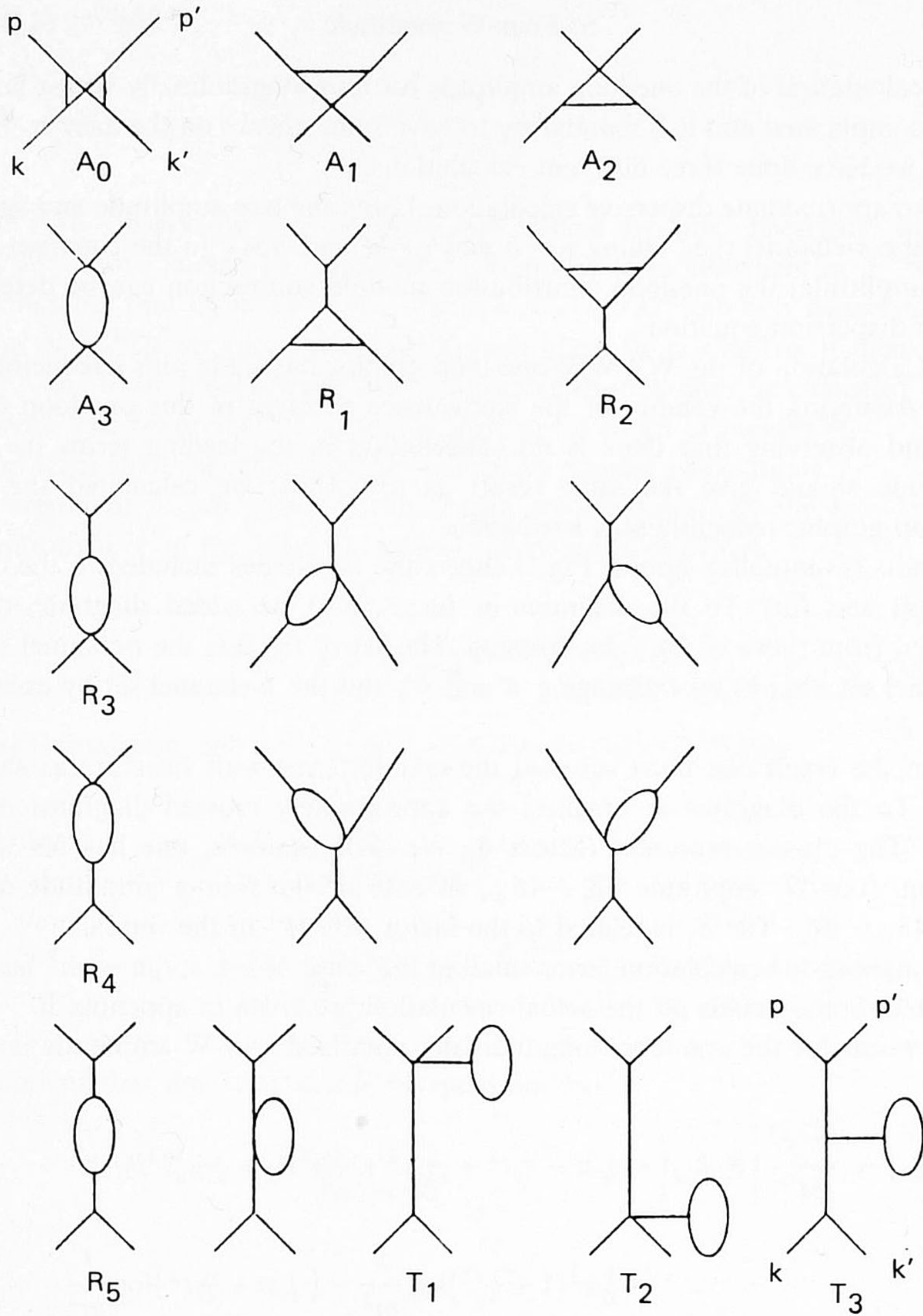
Fig. 3. Topologies of contributing diagrams.
