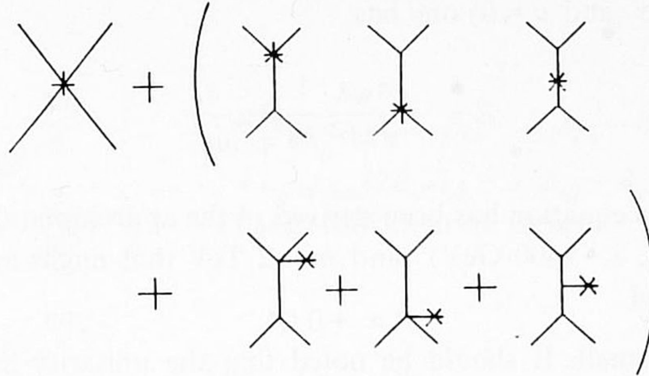
Fig. 4. Structure of counterterms.
