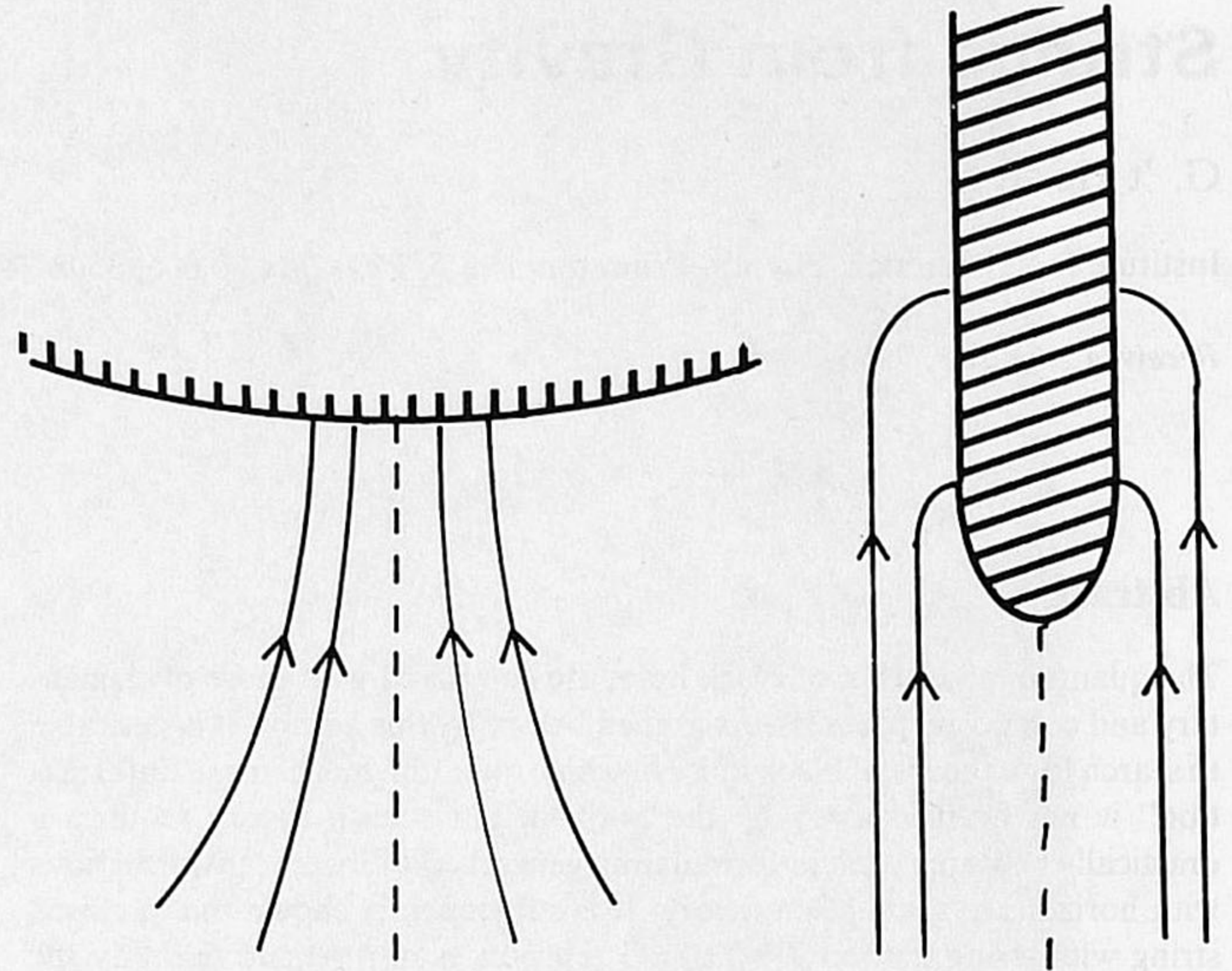
Fig. 3. Coordinate transformations of Fig. 2.
