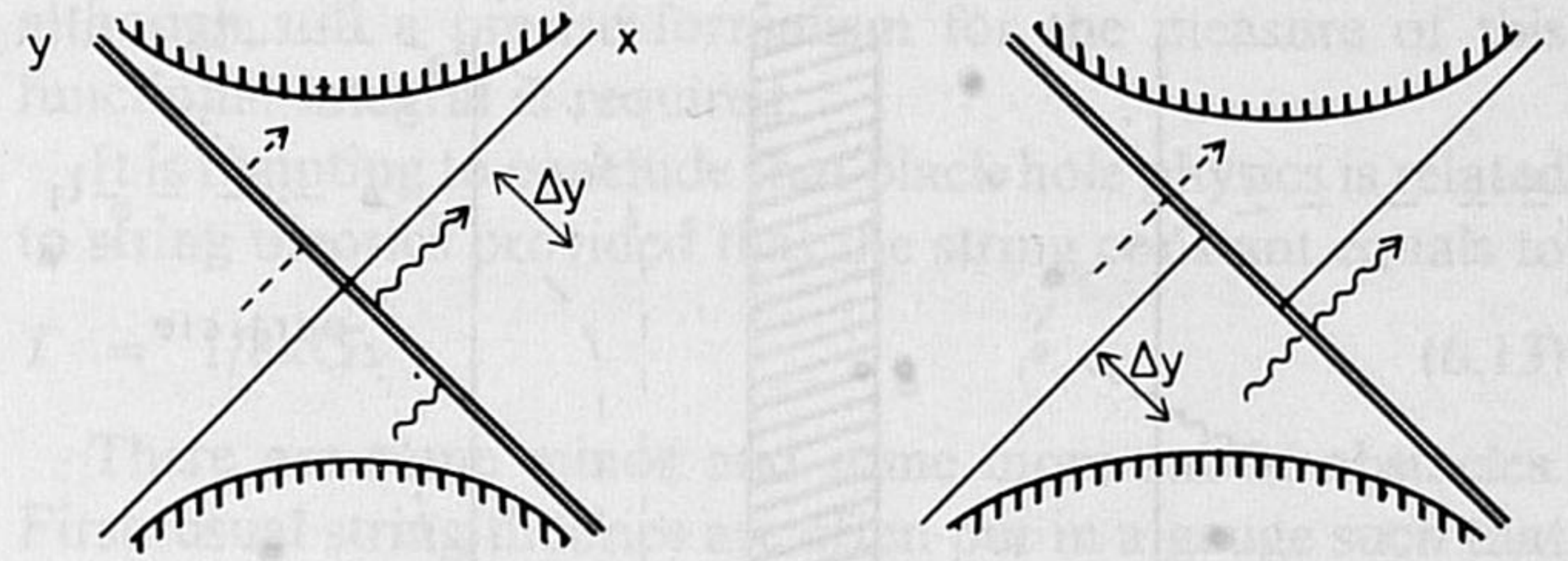
Fig. 8. Change in the metric of a black hole, induced by a single, originally soft particle falling in: (a) Two half Kruskal spaces are connected via a shift. Two geodesics are shown. (b) Coordinates can be deformed such that geodesics are continuous. Future and past horizon are seen not to coincide.
