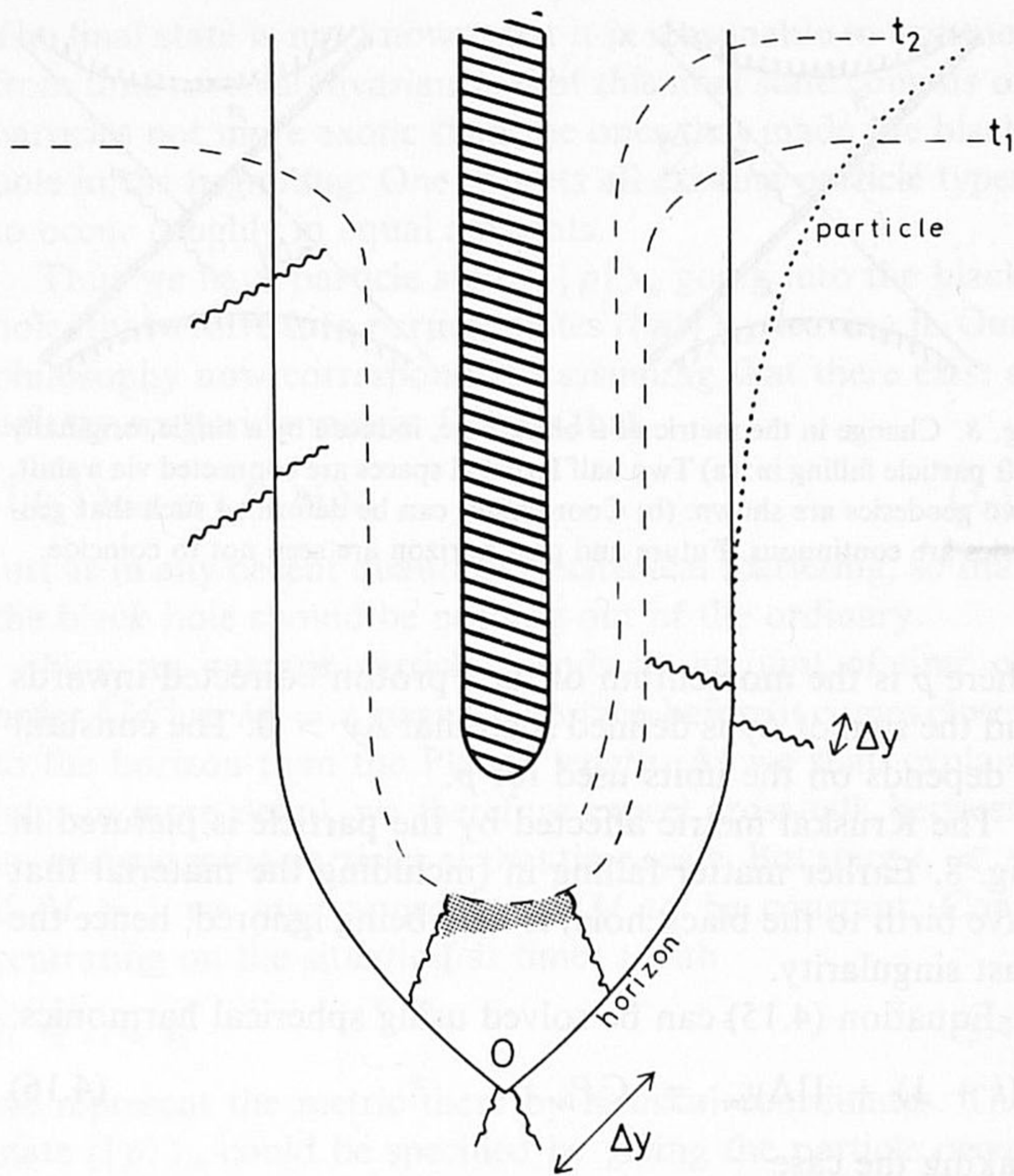
Fig. 9. Soft particles at t_1, t_2 may be hard particles at 0, producing horizon shifts. Some geodesics (wavy lines) are shown.
