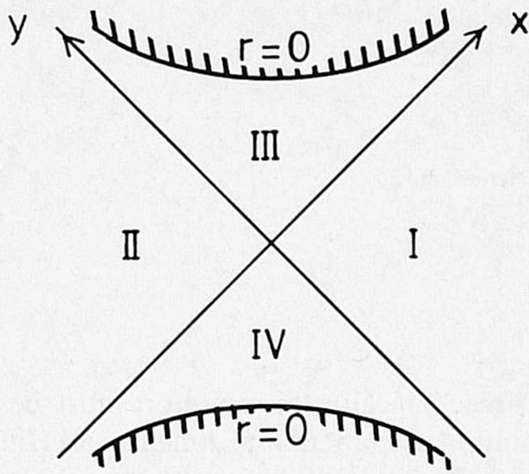
Fig. 1. Schwarzschild black hole in the Kruskal coordinate system.
