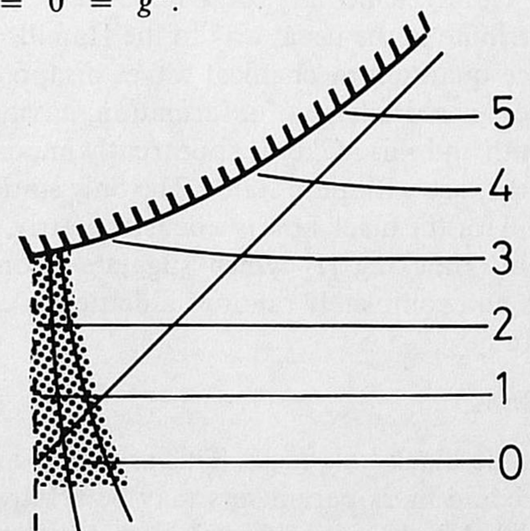
Fig. 4. Time as defined in gauge (2.5).
