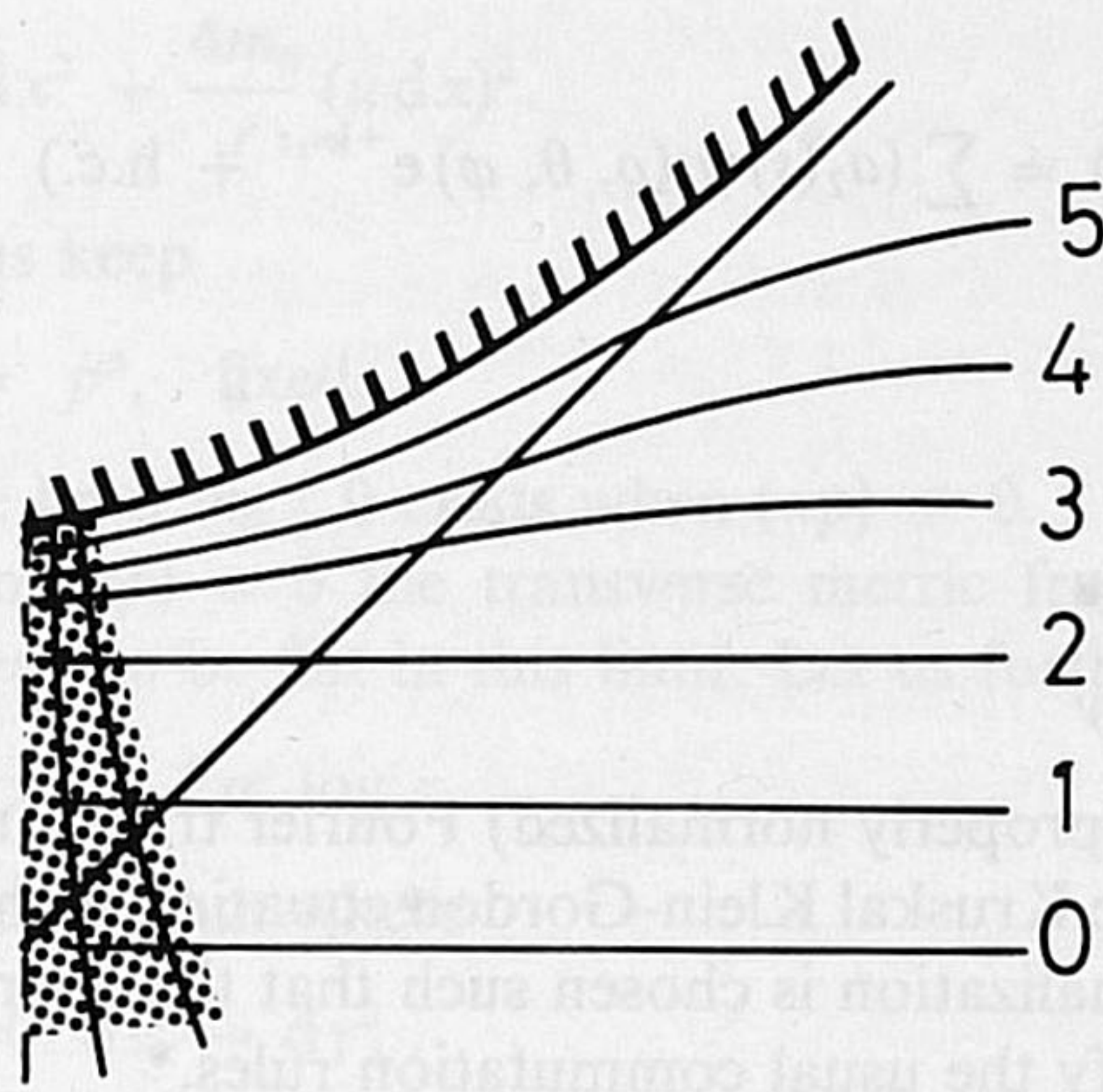
Fig. 5. Time as defined in maximal-volume gauge (2.12).
