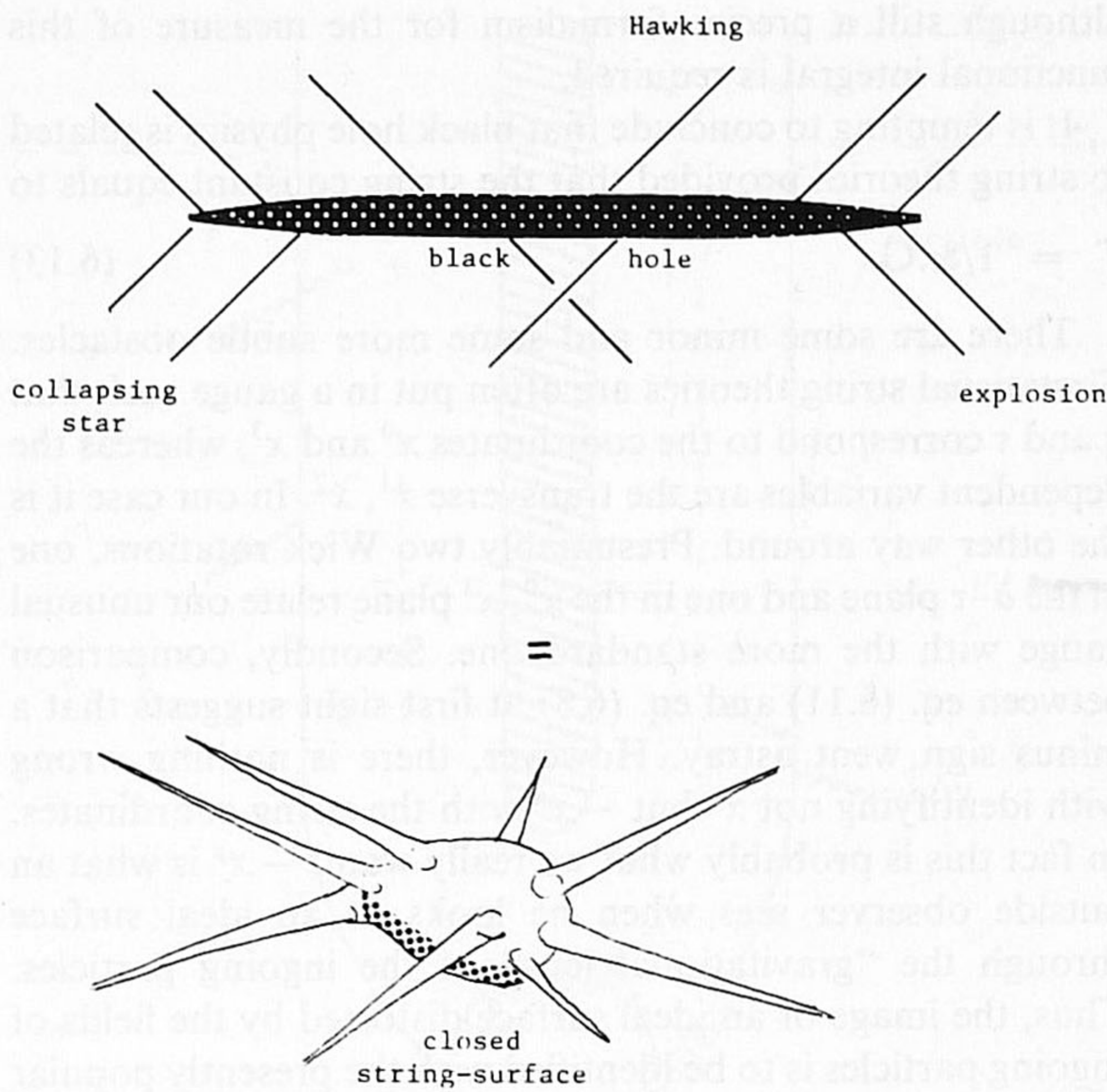
Fig. 10. Formation and destruction of a black hole. Can the amplitudes be obtained from strings theories?
