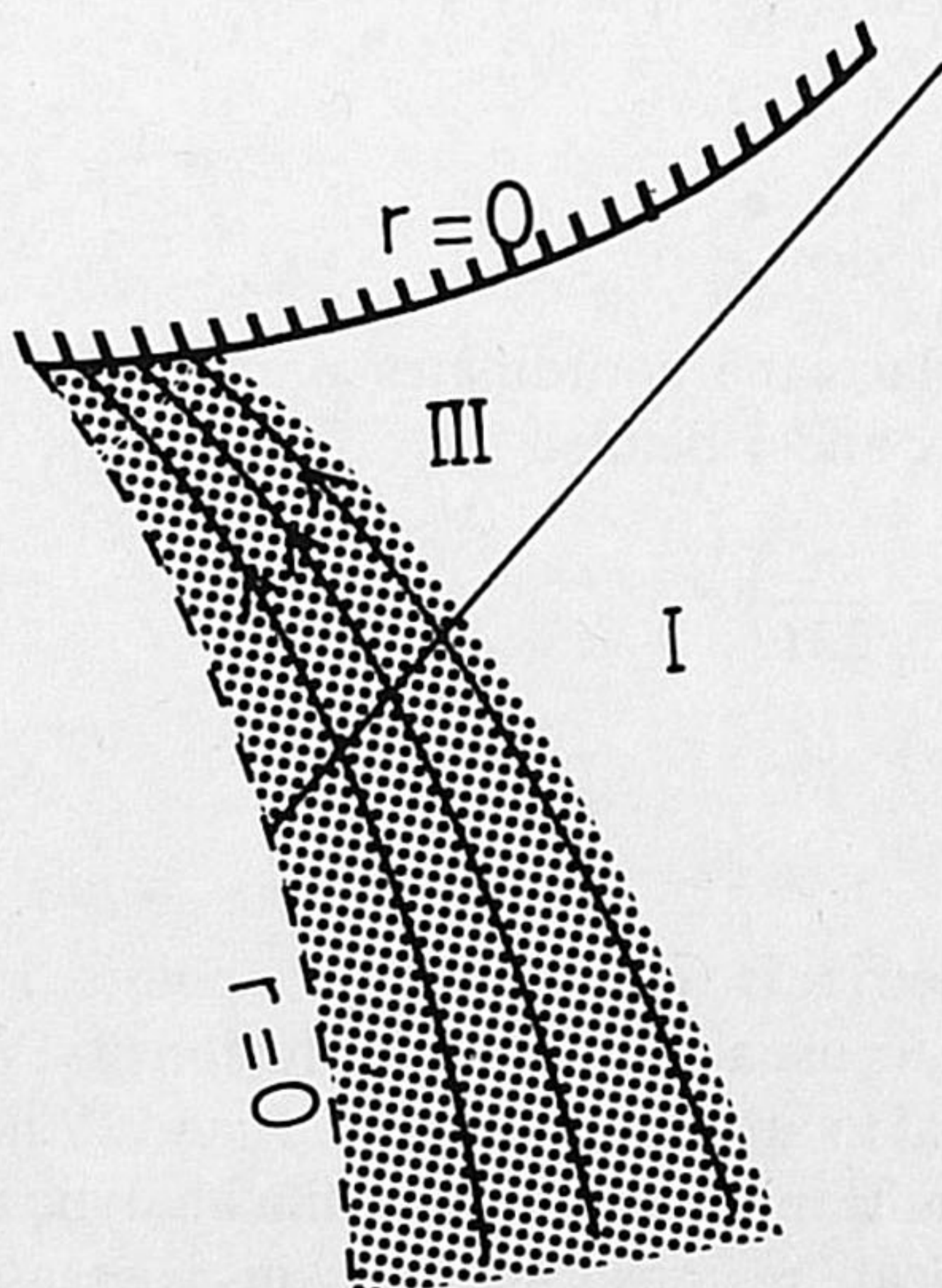
Fig. 2. A physical black hole, including imploding matter, has the Kruskal metric outside, but the regions II and IV are sealed off.
