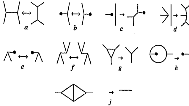
Figure 1. Schematic diagrams of the nine different possible transitions.
