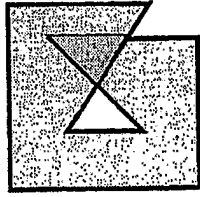
Figure 3. Acceptable self-overlapping polygon.
