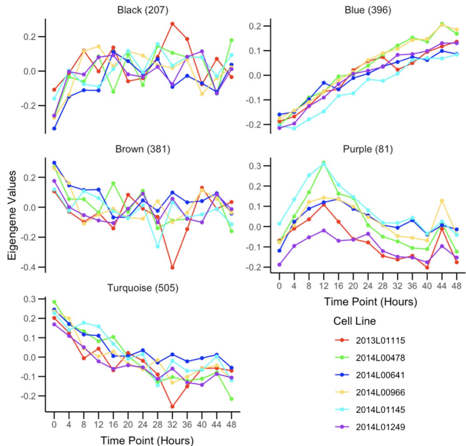
Fig. 1 Eigengene values for RNA-seq modules obtained from WGCNA: Eigengene values of the longitudinal temporal expression patterns of RNA-seq data collected every 4 h for a 48 h period. Each color represents a fibroblast cell culture from a different individual. Module names were assigned by WGCNA. The number of genes assigned per module is indicated next to the module name
