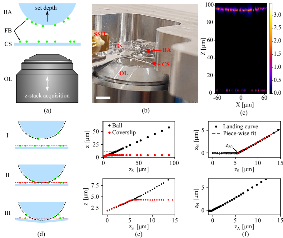
Fig. 4. Experimental setup, and data analysis procedure, used to measure depth-dependent axial scaling. (a) Schematic showing the movable optical objective lens (OL) and sapphire ball (BA) at opposite sides of the static coverslip (CS), with fluorescent beads (FB) on their surfaces. (b) Photograph showing the objective lens (OL), coverslip (CS), and sapphire ball (BA). The ball is glued to a glass strip (GS), which is mounted to the sample shuttle holder (SSH). Scale bar 3 mm. (c) Maximum intensity projection along the Y axis of a recorded z -stack where n_1 = n_2 = 1.0 . The bottom fluorescent signal originates from beads residing on the coverslip, and the signal at the top from beads on the sapphire ball, shown by the visible curvature. (d) Schematic showing three different distances between ball and coverslip, going from clear separation (I) to contact (II) and deformation of the coverslip (III). The dashed lines indicate the position of both ball (red) and coverslip (black). (e) Position of the coverslip and ball versus the set ball-coverslip distance z_S (top) and the same data near the coverslip (bottom). (f) Landing curve (in z_N coordinates), plotted against the set depth z_S (top). The fit values from a piecewise linear fit are used to determine the contact point between ball and coverslip, and this yields the observed focal depth z_N versus the actual depth z_A from which the re-scaling factor \zeta = z_A/z_N was calculated (bottom).
