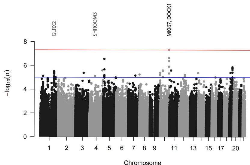
Fig. 1. Manhattan plot of the genome-wide association results. P -values of all tested SNPs on a -\log_{10}(p) scale from the main Cox regression analysis, corrected for genomic inflation. The red line represents the genome-wide significance P -value threshold of 5 \times 10^{-8} , the blue line represents the suggestive threshold of 1 \times 10^{-5} . Genes associated with cardiovascular disease at loci reaching the suggestive threshold or the genome-wide threshold are depicted in grey and black, respectively.
