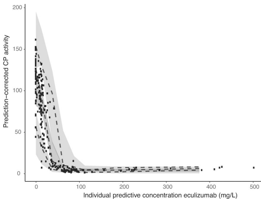
FIGURE 3: Prediction-corrected visual predictive check for the final model. The black dots represent the observed CP activity at corresponding eculizumab concentrations. The dashed lines represent the 5th, median and 95th percentile of the predictions. The majority of the predicted concentrations are in line with the observed concentrations, indicating appropriate validity of the model.
