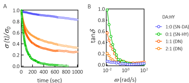
Figure 4. Tunable viscoelastic properties of DN hydrogels. (A) Stress relaxation of different hydrogel formulations after a step strain of \gamma = 2\% (measurements performed on fully cross-linked hydrogels). All hydrogel formulations were prepared at 15 wt % polymer concentration (the mass ratio between DA and HY was varied as indicated, whereas the molar ratios of methylfuran to maleimide and aldehyde to hydrazide were kept at 5:1 and 1:1, respectively). (B) Loss factor \tan \delta , defined as the ratio G''(\omega)/G'(\omega) , as a function of angular frequency (calculated from the corresponding frequency sweep measurements).
