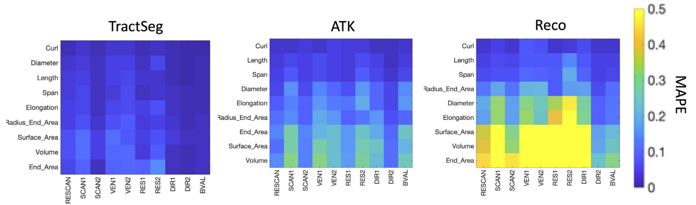
Fig. 7. Variability of shape features is influenced by scanner, vendor, acquisition, and b-value. Variability is shown as MAPE for each TractSeg, ATK, and Reco methods, for scan-rescan (RESCAN), scanners (SCAN1, SCAN2), vendor (VEN1, VEN2), resolution (RES1, RES2), diffusion directions (DIR1, DIR2) and b-value (BVAL). Values shown are averaged across all pathways within a bundle dissection method. Shape features are ordered (from top to bottom) from lowest to highest average MAPE. Many shape features are highly reproducible, and MAPE is influenced by all effects investigated.
