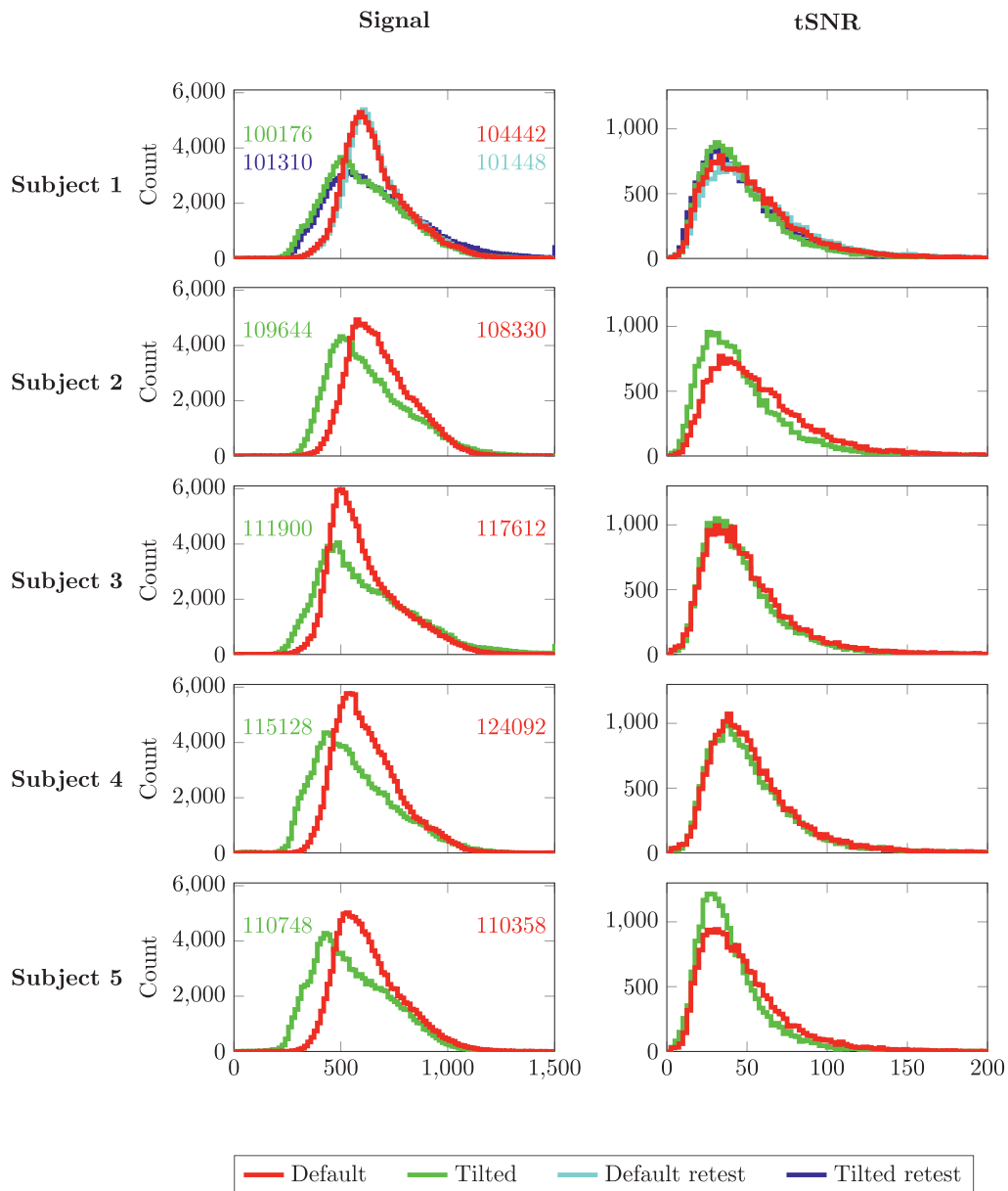
Fig. 3. Distributions of the signal (left column) and temporal SNR (tSNR, right column) in white matter from the data acquired at b = 0\text{s/mm}^2 and TE = 54\text{ ms} in all subjects (rows) for two receive-coil orientations: default in red and tilted in green. For the first subject, default retest (cyan) and tilted retest (blue) signal- and SNR distributions are also shown. Total number of WM voxels for each subject and each head orientation are noted next to the corresponding distribution in the left column.
