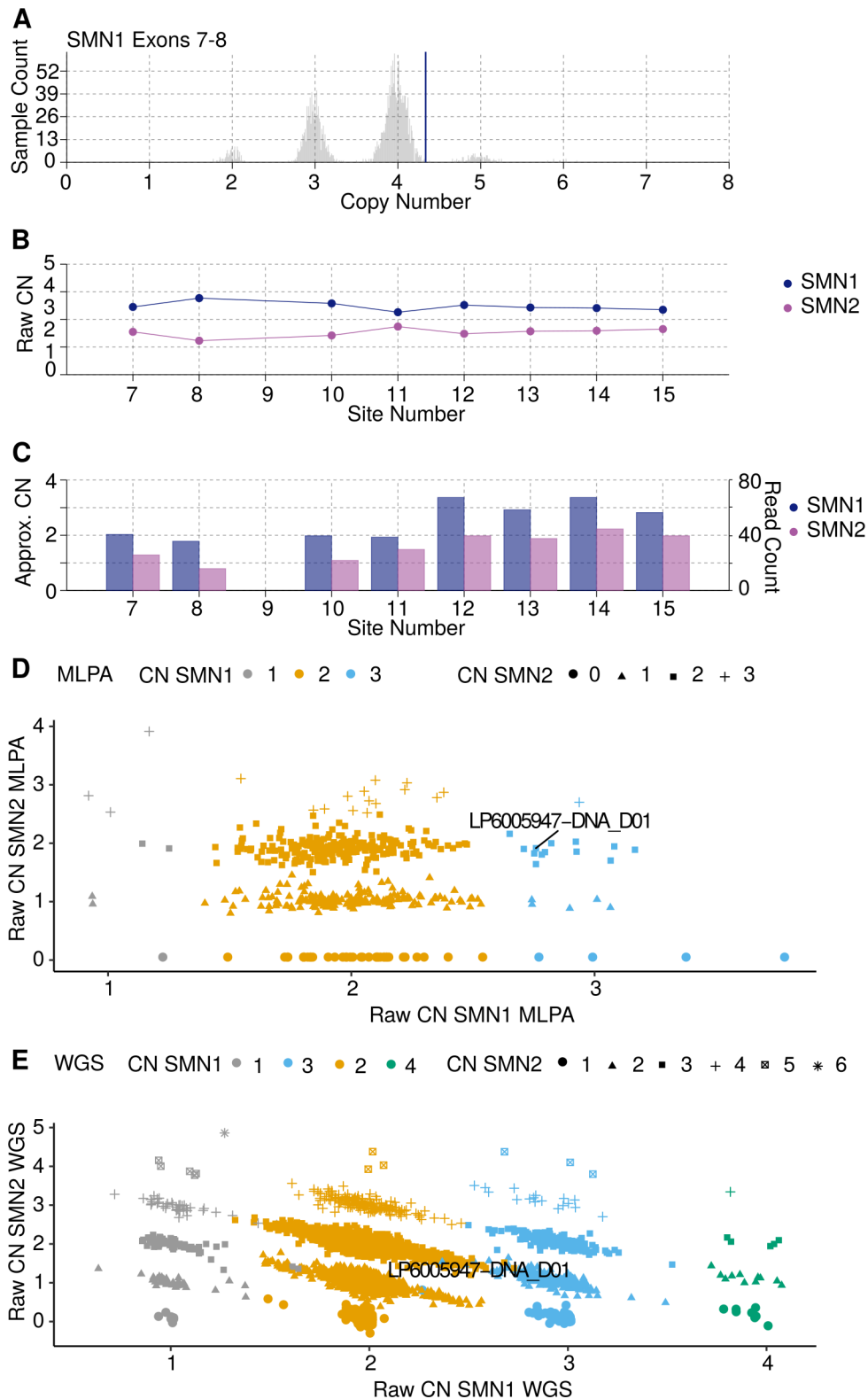
FIGURE 2: Raw data plots for discordant SMNCNC call. MPLA called 3 CNs for SMN1 in sample LP6005947-DNA_D01, whereas SMNCNC called 2 CNs for SMN1 . Closer inspection revealed MLPA to be correct. (A) Raw CN of full length SMN1 estimated by exon 7 and 8, histogram indicating the estimated CN of a large control cohort, vertical blue line indicates the discordant sample. (B) SMN1 and SMN2 raw CN values at the 8 loci used to determine the consensus CN. (C) SMN1 and SMN2 CN normalized against coverage depth at the 8 loci. (D) Scatterplot of the raw CN calls by MLPA, on the x-axis raw CN for SMN1 , and on the y-axis raw CN for SMN2 , discordant sample indicated with a line. (E) Scatter plot of the raw CN calls by SMNCNC, on the x-axis raw CN for SMN1 , and on the y-axis raw CN for SMN2 , discordant sample indicated with a line. CN = copy number; MLPA = multiplexed ligation-dependent probe amplification; SMN = survival of motor neuron; SMNCNC = SMNCopyNumberCaller; WGS = whole genome sequencing.
