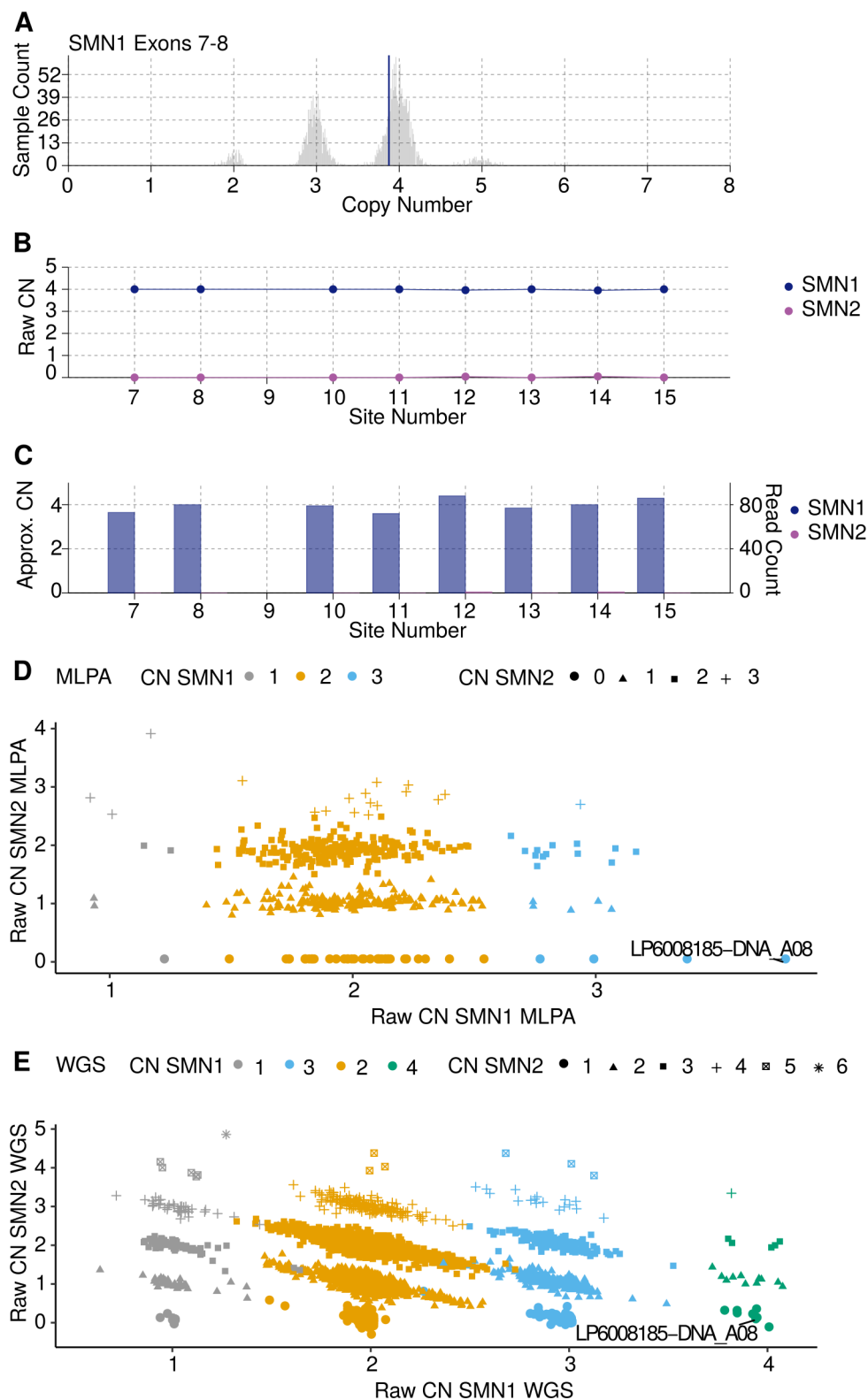
FIGURE 1: Raw data plots for discordant MLPA call. MPLA called 3 CNs for SMN1 in sample LP6008185-DNA_A08, whereas SMNCNC called 4 CNs for SMN1 . Closer inspection revealed SMNCNC to be correct. (A) Raw CN of full length SMN1 estimated by exon 7 and 8, histogram indicating the estimated CN of a large control cohort, vertical blue line indicates the discordant sample. (B) SMN1 and SMN2 raw CN values at the 8 loci used to determine the consensus CN. (C) SMN1 and SMN2 CNs normalized against coverage depth at 8 the loci. (D) Scatterplot of the raw CN calls by MLPA, on the x-axis raw CN for SMN1 , on the y-axis raw CN for SMN2 , discordant sample indicated with a line. (E) Scatter plot of the raw CN calls by SMNCNC, on the x-axis raw CN for SMN1 , and on the y-axis raw CN for SMN2 , discordant sample indicated with a line. CN = copy number; MLPA = multiplexed ligation-dependent probe amplification; SMN = survival of motor neuron; SMNCNC = SMNCopyNumberCaller; WGS = whole genome sequencing.
