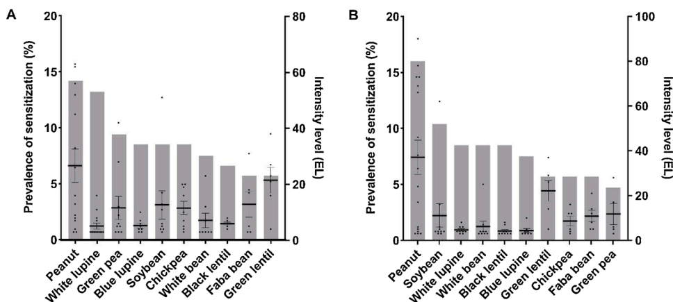
Fig. 2. Sensitization and intensity of IgE binding of 10 legume extracts. The prevalence of sensitization and the intensity of IgE binding for 10 non-processed (A) and processed (B) legume extracts in a suspected food-allergic patient group ( n = 106 ). The prevalence of sensitization (grey bars) is presented as a sample proportion and the intensity of IgE binding (black dots) are presented as the mean \pm SEM.
