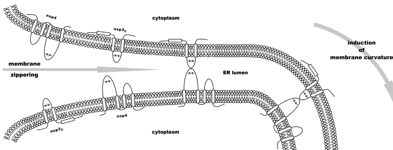
Fig. 8. Model for the interplay between nsp3 and nsp4 in the formation of the CoV replicative structures. The rearrangement of cellular membranes into CoV replicative structures requires the concerted action of both viral and host proteins. We propose that among others the virus contributes to these rearrangements via the expression of nsp3 and nsp4, which interact via their large luminal loops. This interaction “zippers” the ER membranes and induces membrane curvature, two likely requirements for the formation of DMVs that are observed in CoV-infected cells.
