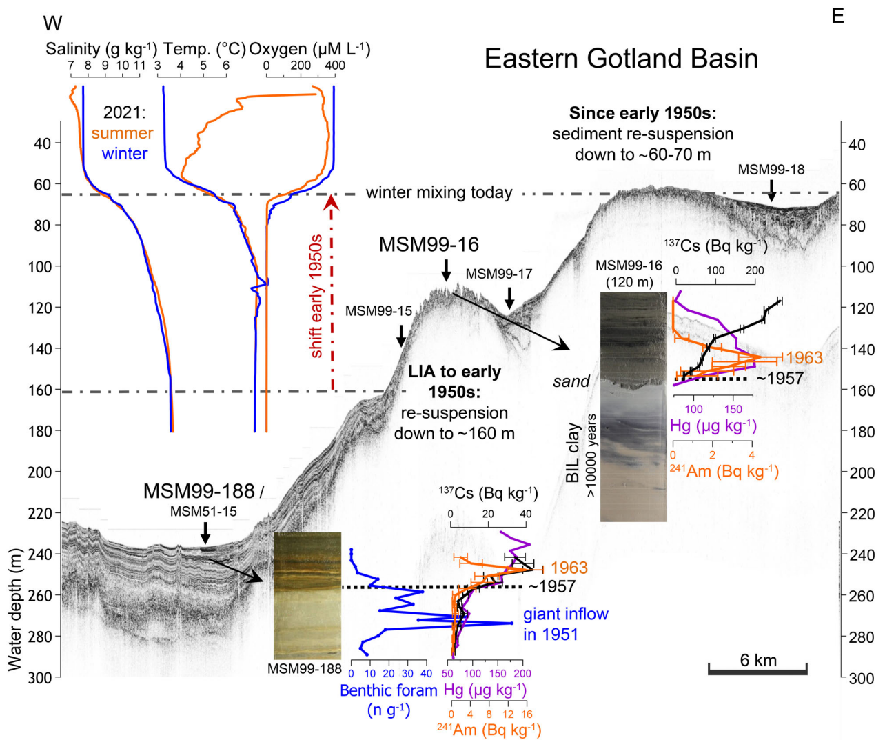
Fig. 4. Hydroacoustic PARASOUND profile from the Eastern Gotland Basin. Subsurface sediment cores were taken on a depths transect from ~240 to 80 m. Stratigraphic markers from two sites bathed at 237 m (MSM99-188 plus benthic foraminiferal counts) and 120 m (MSM99-16) water depth, respectively, are shown. Note that the environmental and sedimentological (dashed horizontal line ~1957) change occurred shortly after the giant saline inflow in 1951 (numerically massive appearance of benthic foraminifera). Since the mid-1950s calmer conditions have enabled the accumulation of organic-carbon-rich material also in shallower areas up to the modern winter-time mixing depth of 60–70 m (see summer and winter CTD data upper left). Time marker: AD 1963 nuclear weapons test maximum.
