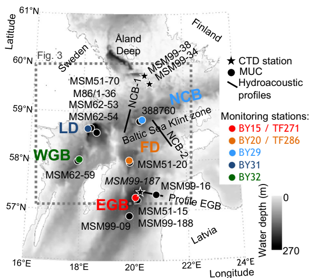
Fig. 1. Bathymetric map showing the various sub-basins (WGB = Western Gotland Basin; EGB = Eastern Gotland Basin; FD = Fårö Deep; NCB = Northern Central Basin; LD = Landsort Deep) of the Baltic Proper and key multi-core (black dots), CTD (asterisk) and hydrographic monitoring (coloured dots) stations. Black bold lines indicate locations of hydroacoustic profiles and the box marked with a dashed grey line displays the map area shown in Fig. 3. The topographic barrier named 'Baltic Sea Klint' is indicated. Locations of additional multi-cores are not shown in this figure but are revealed in the respective hydroacoustic profiles (Figs 4, S3–S5).
