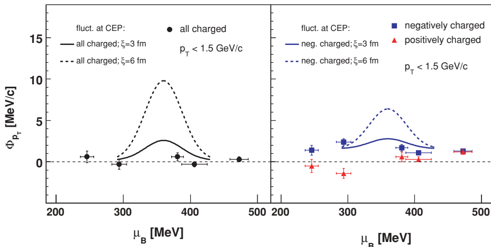
FIG. 20. (Color online) \Phi_{p_T} as a function of baryochemical potential ( \mu_B values from statistical hadron gas model fits [32]) for the 7.2% most central Pb + Pb interactions. Results with p_T < 1.5 GeV/c (as in Fig. 12). Data (points) are corrected for limited two-track resolution. Errors are statistical only. The Gaussian curves show estimated \Phi_{p_T} values in the case of the existence of the critical point (see text for details).
