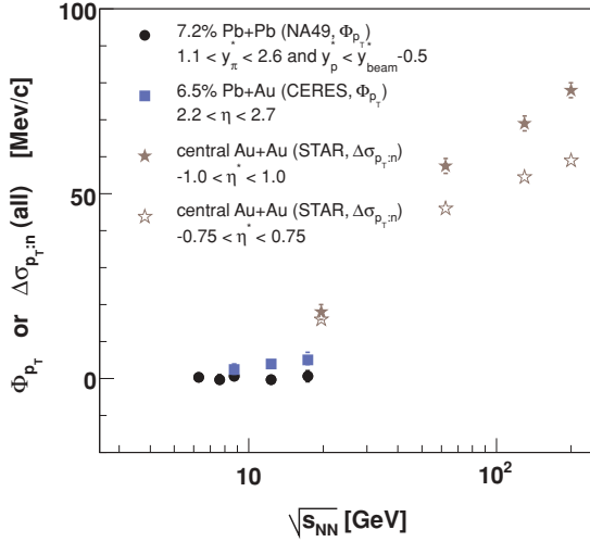
FIG. 23. (Color online) \Phi_{p_T} or \Delta\sigma_{p_T:n} as a function of energy measured for all charged particles by the NA49, CERES, and STAR experiments. The NA49 points are obtained for the forward-rapidity region in a limited azimuthal angle acceptance; the CERES [16] and STAR (Fig. 3, left, in Ref. [35]) points are calculated for midrapidity regions within complete azimuthal acceptances. All data points include small-scale correlations (HBT, etc.). STAR data are corrected for tracking inefficiency.
