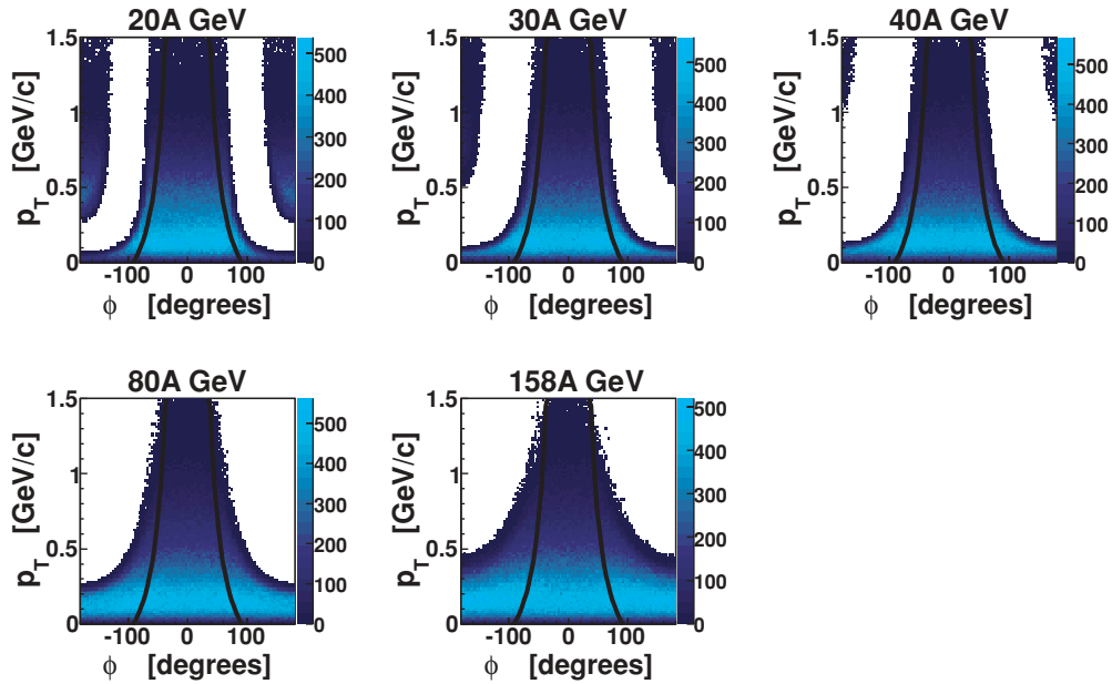
FIG. 2. (Color online) NA49 (\phi, p_T) acceptance of all charged particles for 2.0 < y_\pi^* < 2.2 . Additional cut on y_p^* (see the text) is not included. The solid lines represent the analytical parametrization of the common acceptance.
