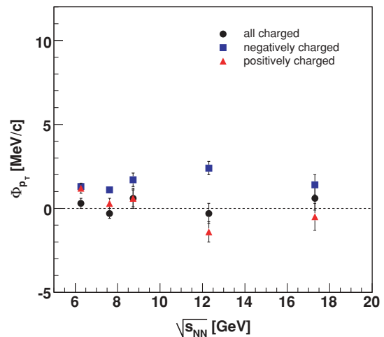
FIG. 12. (Color online) \Phi_{p_T} as a function of energy for the 7.2% most central Pb + Pb interactions. Data points are corrected for limited two-track resolution. Errors are statistical only. Systematic errors are given in Table IV.
