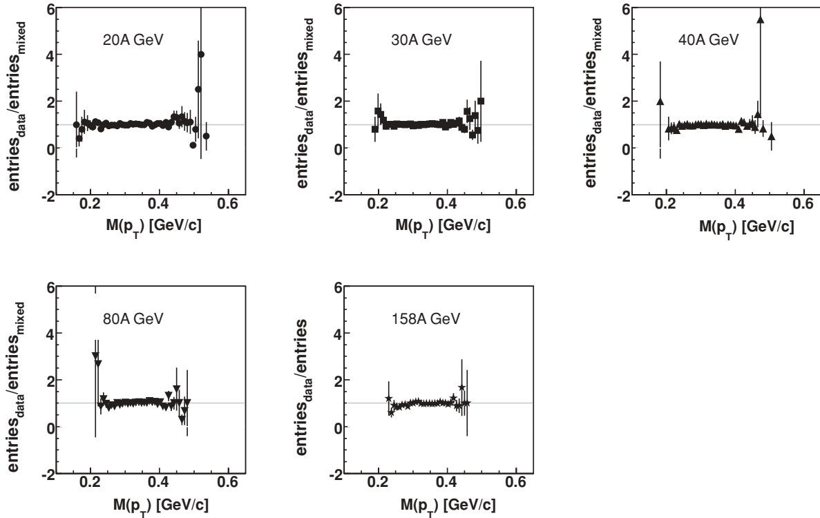
FIG. 11. Distributions of mean transverse momentum for data divided by distribution for mixed events (see the previous figure).
