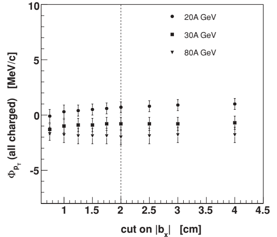
FIG. 6. Dependence of \Phi_{p_T} on upper cut in the impact parameter |b_x| . For each point, the cut on |b_y| is equal to half the cut on |b_x| . Note: the values and their errors are correlated. The dashed line indicates the cut used in the analysis.
