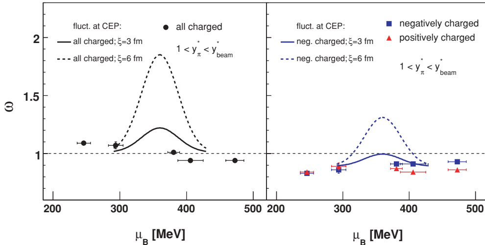
FIG. 21. (Color online) \omega [6] as a function of baryochemical potential ( \mu_B values from statistical hadron gas model fits [32]) for the 1% most central Pb + Pb interactions in 1 < y_\pi^* < y_{\text{beam}}^* . Errors are statistical only. The Gaussian curves show estimated \omega values in the case of the existence of the critical point (see text for details).
