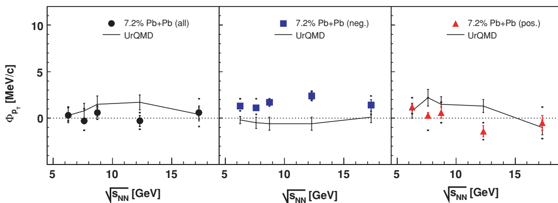
FIG. 16. (Color online) Comparison of \Phi_{p_T} as a function of energy from data (data points, corrected for limited two-track resolution) with UrQMD model calculations (black lines) with acceptance restrictions as for the data. The panels represent results for all charged (left), negatively charged (center), and positively charged particles (right).
