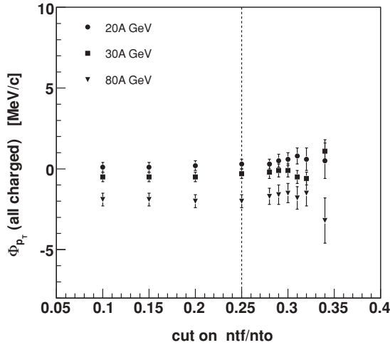
FIG. 4. Dependence of \Phi_{p_T} on one of the event cuts (ntf/nto ratio). Note: the values and their errors are correlated. The dashed line indicates the cut used in the analysis.
