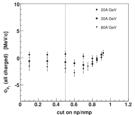
FIG. 7. Dependence of \Phi_{p_T} on lower cut on np/nmp ratio. Note: the values and their errors are correlated. The dashed line indicates the cut used in the analysis.
