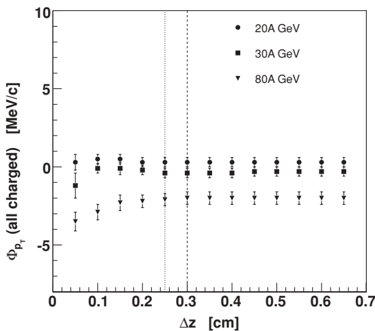
FIG. 5. Dependence of \Phi_{p_T} on the allowed distance \Delta z from the nominal position of the main vertex. Note: the values and their errors are correlated. The dashed line indicates the cut used in the analysis of 30A and 80A GeV data. The dotted line represents the cut used in the analysis of 20A GeV data.
