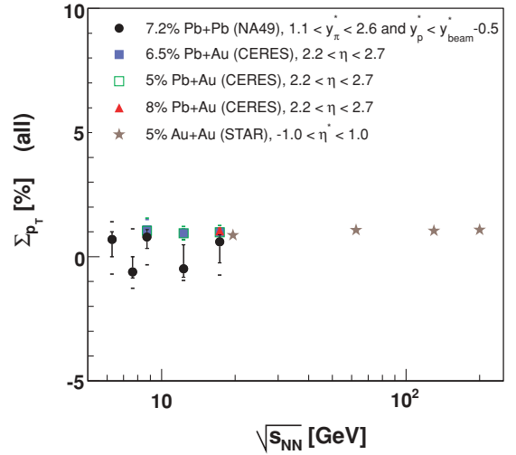
FIG. 25. (Color online) \Sigma_{p_T} (%) as a function of energy measured for all charged particles by the NA49, CERES, and STAR experiments. The NA49 points are obtained for the forward-rapidity region in a limited azimuthal angle acceptance; the CERES [16] (point for 8% most central Pb + Au collisions taken from Ref. [25]) and STAR [36] points are calculated for midrapidity regions within complete azimuthal acceptances.
