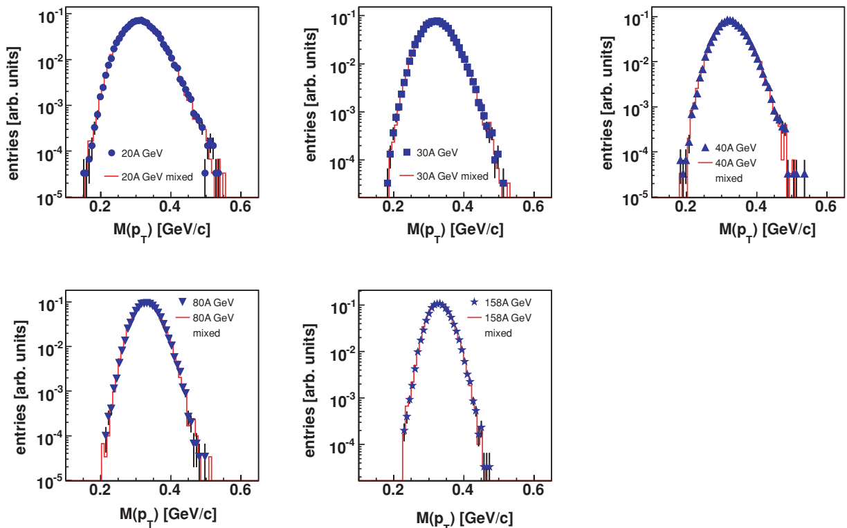
FIG. 10. (Color online) Distributions of mean transverse momentum for data (points) and mixed events (histograms). Data points are not corrected for acceptance and limited two-track resolution. Events with accepted particle multiplicity equal to zero are not used.
