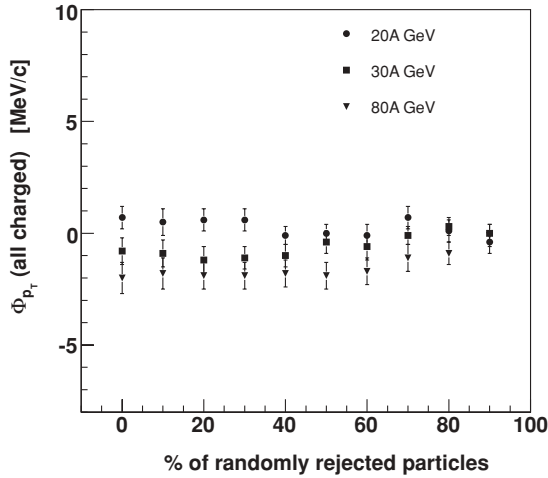
FIG. 9. Dependence of \Phi_{p_T} on the fraction of randomly rejected particles.
