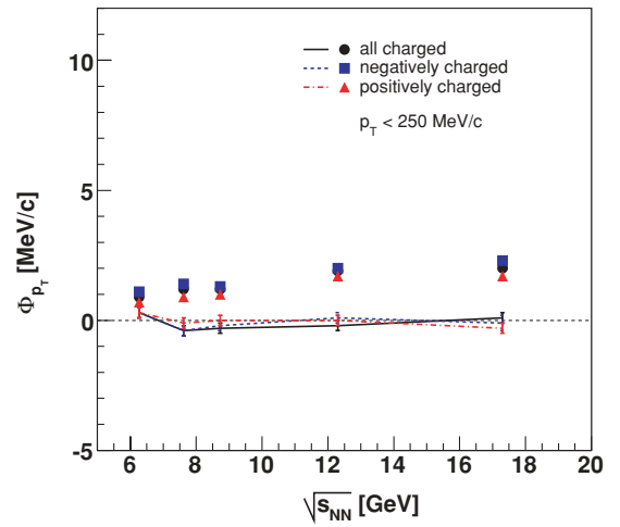
FIG. 19. (Color online) Same as Fig. 17, but with additional cut p_T < 250 MeV/c.
