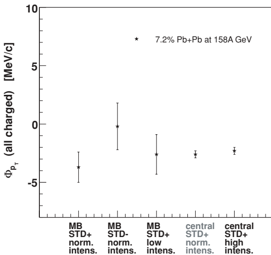
FIG. 8. \Phi_{p_T} values for different central and minimum-bias (MB) data sets. Data used for the further analysis are central STD+ normal intensity.
