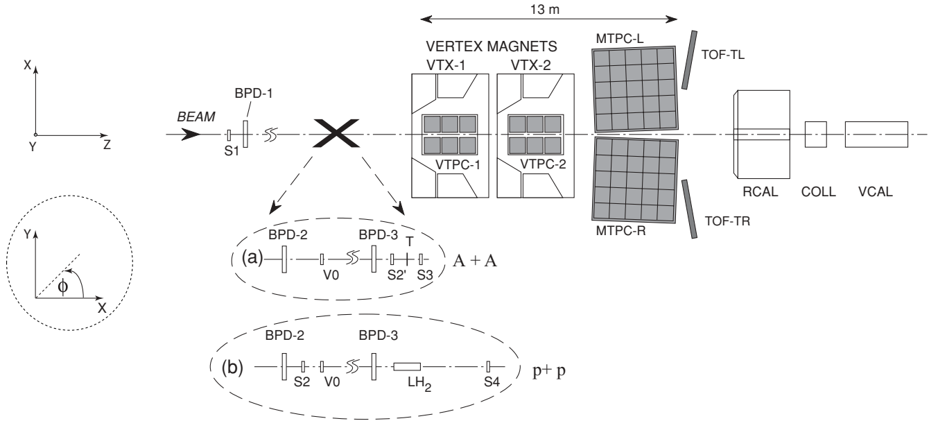
FIG. 1. Experimental setup of the NA49 experiment [20] with different beam definitions and target arrangements.
