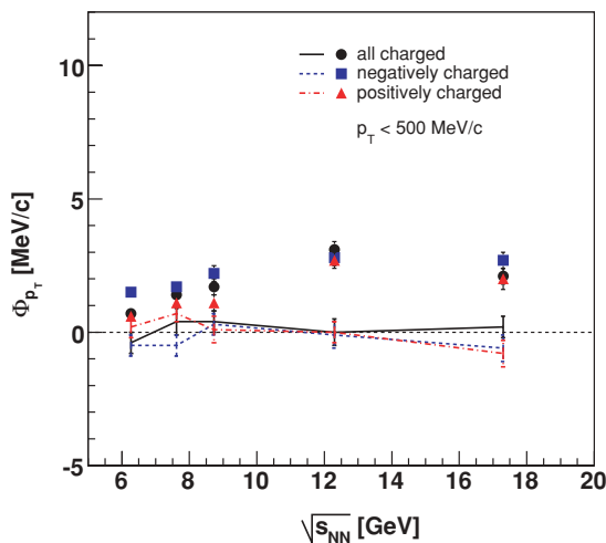
FIG. 18. (Color online) Same as Fig. 17, but with additional cut p_T < 500 MeV/c.
