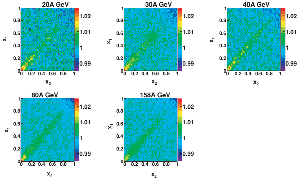
FIG. 13. (Color online) Two-particle correlation plots (x_1, x_2) using the cumulant p_T variable x . The bin contents are normalized by dividing with the average number of entries per bin. Plots are for all charged particles for central Pb + Pb collisions at 20A–158A GeV. Note that the color scale is the same in all panels.
