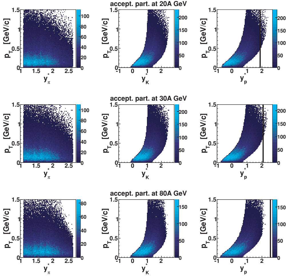
FIG. 3. (Color online) (y^*, p_T) plots of all accepted (see Fig. 2) particles assuming pion (left), kaon (middle), and proton (right) mass. Additional cut on y_p^* (see the text) is not included. Top, middle, and bottom panels correspond to 20A, 30A, and 80A GeV data, respectively. Black lines represent beam rapidities ( y_{\text{beam}}^* ) in the center-of-mass reference system.
