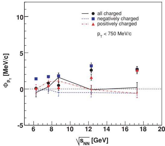
FIG. 17. (Color online) \Phi_{p_T} as a function of energy for the 7.2% most central Pb + Pb interactions, with additional cut p_T < 750 MeV/c. Data (points) are corrected for limited two-track resolution. Lines show results of UrQMD calculations with the same kinematic and acceptance restrictions. Errors are statistical only.
