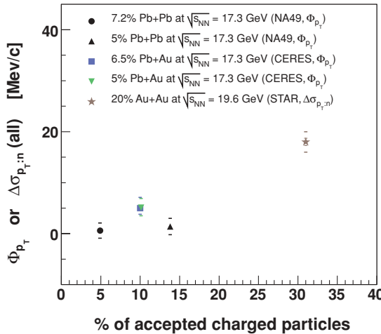
FIG. 24. (Color online) \Phi_{p_T} or \Delta\sigma_{p_T:n} as a function of percent of charged particles accepted in the analysis. Data are presented for the top SPS and the lowest RHIC energies. The NA49 points (Ref. [10] and this analysis) are obtained for the forward-rapidity region in a limited azimuthal angle acceptance; the CERES [16] and STAR [35] points are calculated for midrapidity regions within complete azimuthal acceptances. All data points include small-scale correlations (HBT, etc.).
