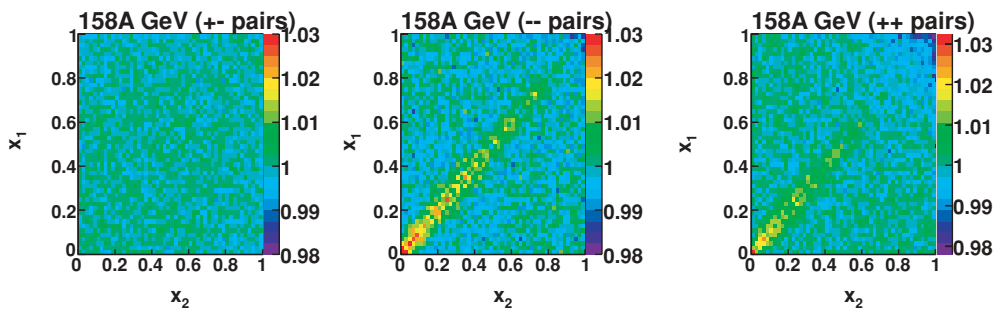
FIG. 15. (Color online) Two-particle correlation plots (x_1, x_2) using the cumulant p_T variable x . The bin contents are normalized by dividing with the average number of entries per bin. Plots are for central Pb + Pb collisions at 158A GeV for unlike-sign particles (+-), and for negatively and positively charged particles, separately. Note that the color scale can be slightly different for different panels.
