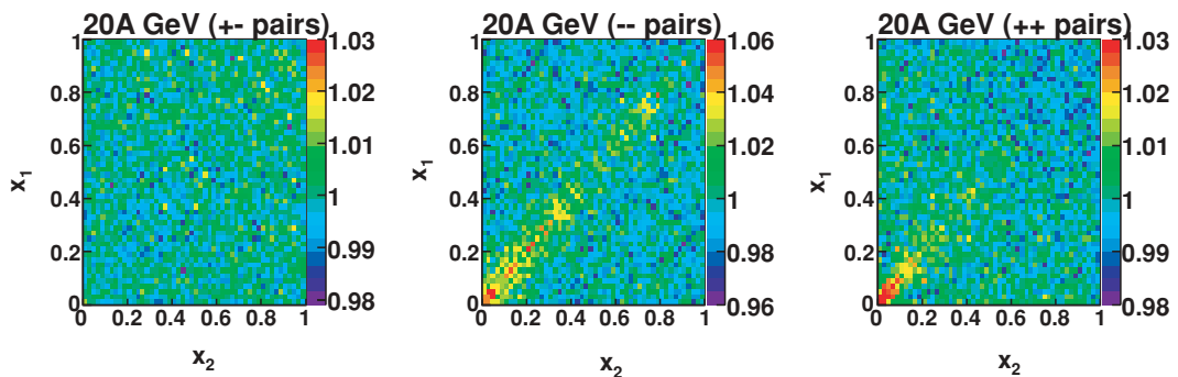
FIG. 14. (Color online) Two-particle correlation plots (x_1, x_2) using the cumulant p_T variable x . The bin contents are normalized by dividing with the average number of entries per bin. Plots are for central Pb + Pb collisions at 20A GeV for unlike-sign particles (+-) , and for negatively and positively charged particles, separately. Note that the color scale can be slightly different for different panels.
