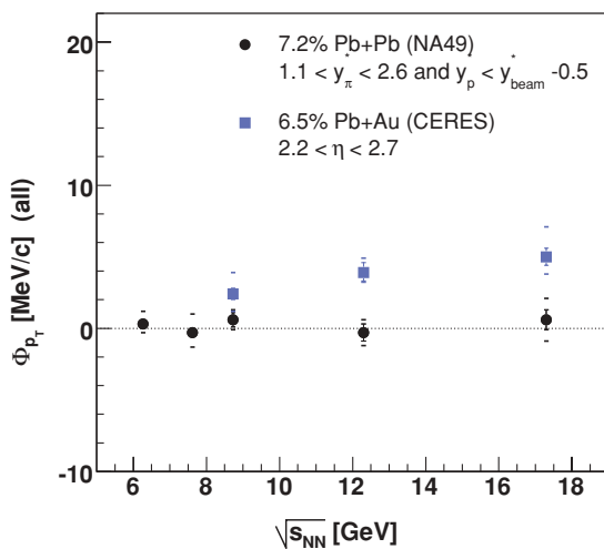
FIG. 22. (Color online) \Phi_{p_T} as a function of energy measured for all charged particles by the NA49 and CERES experiments. The NA49 points are obtained for the forward-rapidity region in a limited azimuthal angle acceptance; the CERES data [16] are calculated for the midrapidity region within a complete azimuthal acceptance. All data points include small-scale correlations (HBT, etc.).
