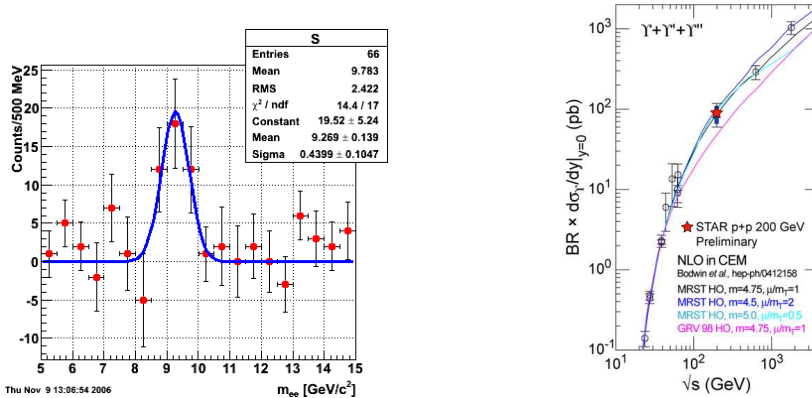
Figure 2: Left panel: Background subtracted di-electron invariant mass distribution in p+p collisions at \sqrt{s_{NN}} = 200 GeV. The blue line indicates a Gaussian fit to the data. Right panel: Excitation function of the \Upsilon cross section. The data is compared to previous measurements and NLO calculations. The curves of the NLO calculations are scaled by a factor of 1.44 to account for the excited states.
