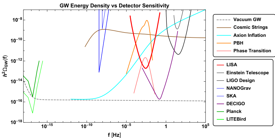
Fig. 5 SGWB energy density h^2\Omega_{\text{GW}} for different cosmological sources compared to the sensitivity of different GW detectors. As cosmological signals we have the vacuum GW contribution coming from inflation (grey dashed line) with r = 0.044 and n_T = -r/8 , the signal expected in axion inflation models (cyan), the signal generated by cosmic string networks with G\mu = 10^{-10} (brown), the signal generated by a FOPT with v_w = 0.9 , \alpha = 0.1 , \beta/H_* = 50 , g_* = 100 , T_* = 200\text{GeV} (pink) and the signal generated at second-order by the formation mechanism of PBHs with f_{\text{PBH}} = 1 , \sigma = 0.5 , k_* = k_{\text{LISA}} (orange). For GW detectors we report the sensitivity of Planck (darker green), LITEBird (green), EPTA (blue), SKA (darker blue), LISA (red), DECIGO (purple), LIGO Design (black) and ET (darker black)
