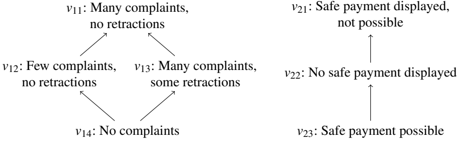
Figure 1. Hesse diagrams for the \geq_{\text{PRO}} ordering of the two dimensions in (a toy example version of) the web shop domain \{d_1, d_2\} . The dimension d_1 , displayed on the left, has the four values \{v_{11}, v_{12}, v_{13}, v_{14}\} while dimension d_2 , on the right, has three values \{v_{21}, v_{22}, v_{23}\} . If there is a path from value a to b then a \geq_{\text{PRO}} b .
