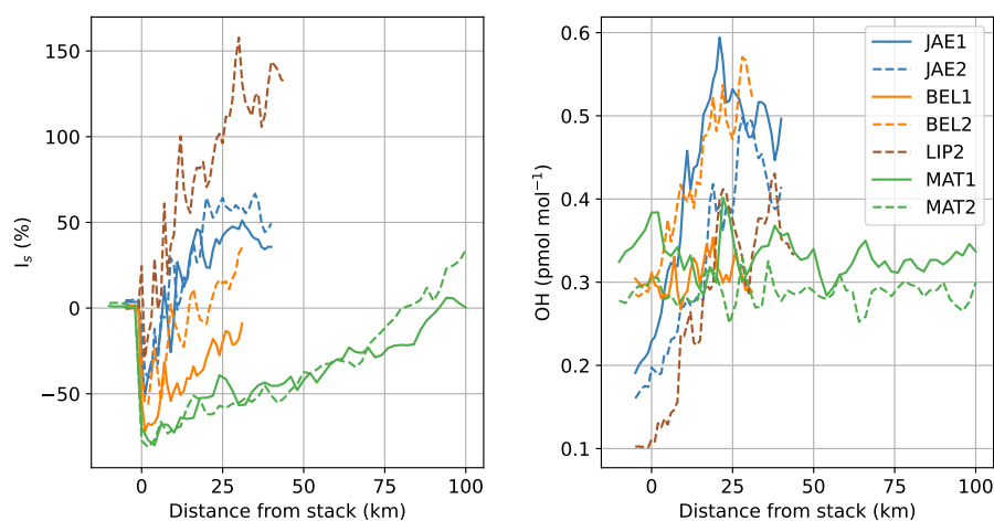
Figure 7. I s,NO 2 ,OH (in percent) and mean OH (in pmol mol -1 ) as a function of distance from the stack location. Leftmost x-values smaller than zero represent background air. For definition of the volumes that were used for averaging, see Fig. 6. I s is defined in Eq. 6.
