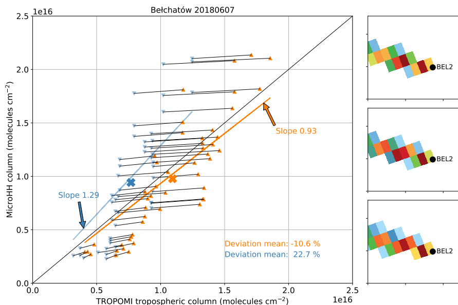
Figure 11. Comparison of simulated and TROPOMI tropospheric \text{NO}_2 columns for simulation BEL2. The three simulated plumes shown in the rightmost panels are 15 minutes apart around TROPOMI overpass time and are used to account for variations in the turbulent field. Domain and color bar as in Fig. 2, but in the range 0\text{--}2 \times 10^{16} molecules \text{cm}^{-2} . These fields are coarsened to TROPOMI resolution and filtered for enhanced \text{NO}_2 mixing ratios to identify the plume (see text). The blue dots and line show comparisons for TROPOMI data that have not been corrected for the AMF (Eq. 4). Moreover, simulated profiles have not been augmented with CAMS \text{NO}_2 in the free troposphere (i.e. 0\text{--}4 km). The orange dots show the corrected and augmented values, with corrected (orange) and uncorrected (blue) points connected by thin grey lines. Orange and blue lines and slope values represent fits that are forced through the origin. The orange and blue crosses represent the plume-mean columns and mean deviations ( (\text{model}-\text{tropomi})/\text{tropomi} in %) are given in the lower right corner.
